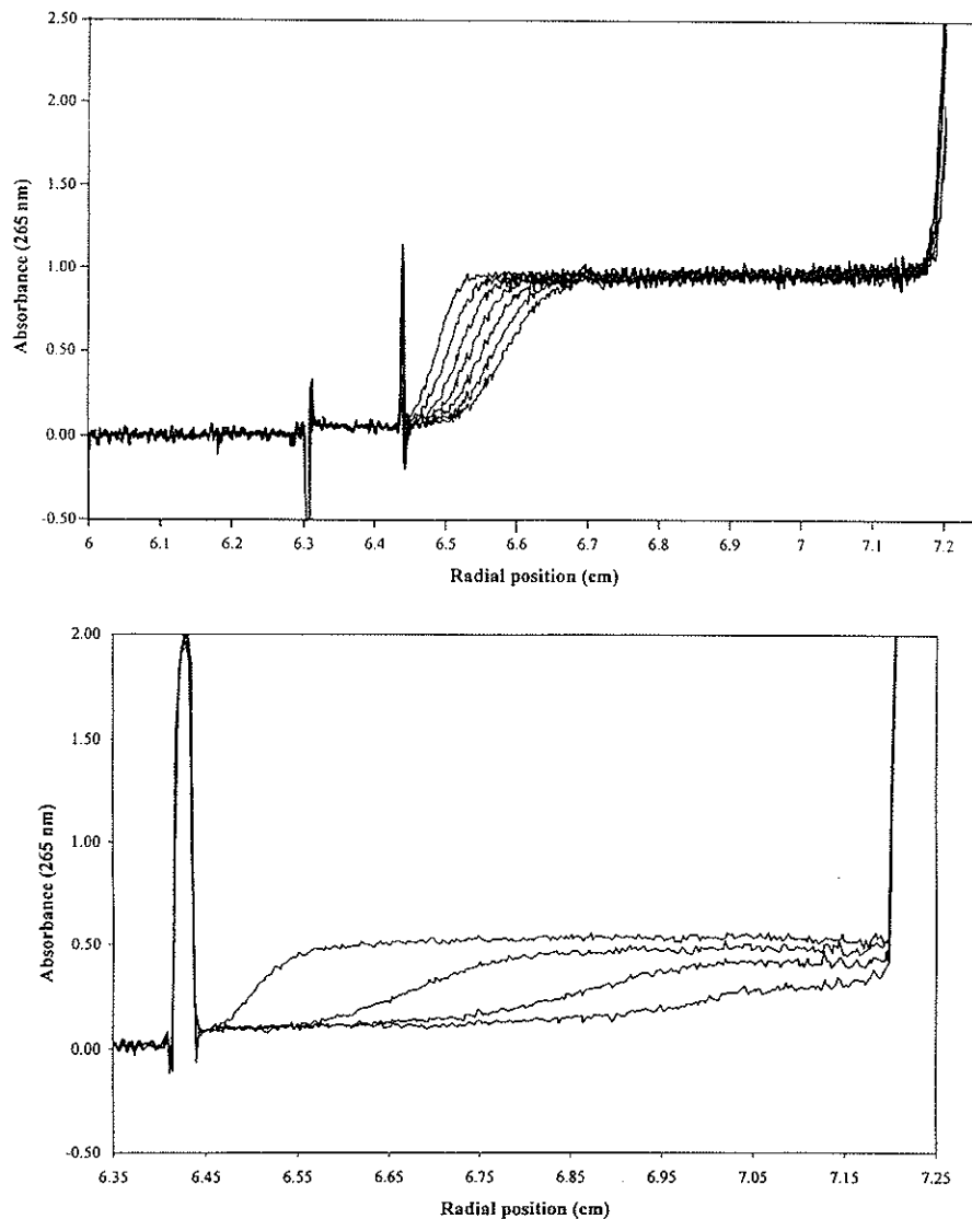
Figure 13. Sedimentation velocity analysis demonstration of mucoadhesion of the mussel glue protein mefp-1 with pig gastric mucin. XL-A analytical ultracentrifuge used equipped with scanning uv-absorption optics (a) mefp-1 control. Rotor speed = 40,000 rev/min, temperature = 20.0°C, scan interval = 10 min, loading concentration = 0.8mg/ml. Sedimentation coefficient, s_{20} = (2.34 \pm 0.17)S . (b) mefp-1 : mucin complex (Concentration of mucin after mixing = 0.1 mg/ml; concentration of mefp-1 after mixing = 0.4 mg/ml. Rotor speed = 2,000 rev/min, temperature = 20.0°C, scan interval = 10 min, s_{20} \sim 7000S . (From Deacon et al. , 1998).
