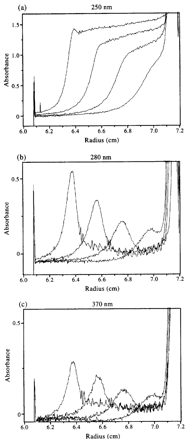
Fig. 2. Sedimentation velocity diagrams for Chitosan 2 ( F_A = 0.61 ) from the absorption optical system of the XL-A ultracentrifuge. (a) wavelength = 250 nm (b) wavelength = 280 nm (c) wavelength = 370 nm. Degree of substitution = 1%. Rotor speed = 50,000 rev/min, temperature = 20°C, loading concentration = 2 mg/ml, scan interval = 120 min. Direction of sedimentation is from left to right.
