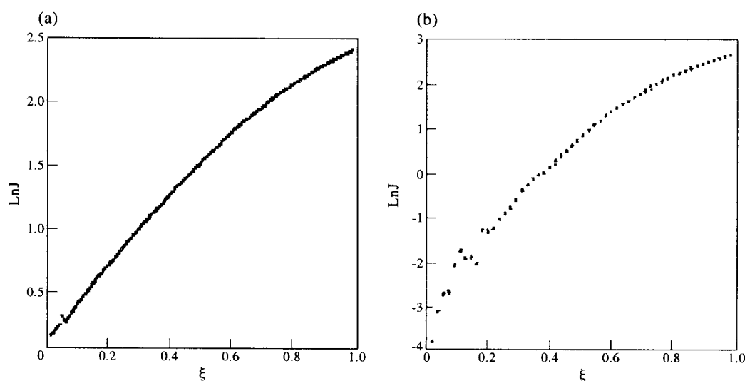
Fig. 5. Plot of the logarithm of the fringe displacement, J versus the normalised radial displacement squared parameter, \xi , at a loading concentration of 2.0 mg/ml. \xi = (r^2 - a^2)/(b^2 - a^2) where r is the radial displacement from the centre of the rotor of a given point in the ultracentrifuge cell, and a and b the corresponding radial positions of the solution/air meniscus and the cell base respectively. (a) chitosan 1, DS = 0.01%, rotor speed = 18 000 rev/min. (b) chitosan 2, DS = 0.01%, rotor speed = 18 000 rev/min.
