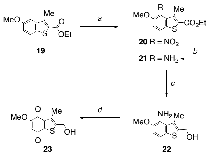
Scheme 4. Reagents and conditions: a, HNO 3 , AcOH, rt (74%); b, Sn, HCl, EtOH, reflux (86%); d, LiAlH 4 , THF, rt (80%); d, Fremy's salt, NaH 2 PO 4 , aq acetone, rt (67%).
