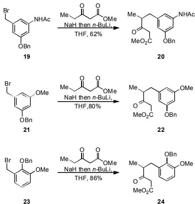
Scheme 4. Preparation of 5-aryl-3-oxopentanoate oxidative cyclization precursors.
