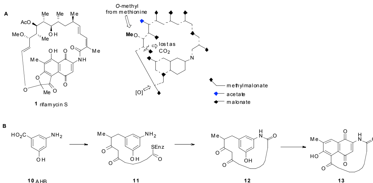
Scheme 2. A, The results of labelling studies carried out on rifamycin S; B, Rickards' biosynthetic proposal for the naphthoquinone ansamycins.
