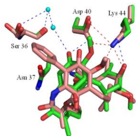
Fig. 2 X-ray structure of 19-phenyl geldanamycin 5 bound in the ATP site of yeast Hsp90.11 Geldanamycin 1 (green) and 19-phenyl geldanamycin 5 (salmon) with Hsp90 (green and salmon residues, respectively). See PDB codes 1A4H (geldanamycin 1) and 4ASF (19-phenyl geldanamycin 5).
