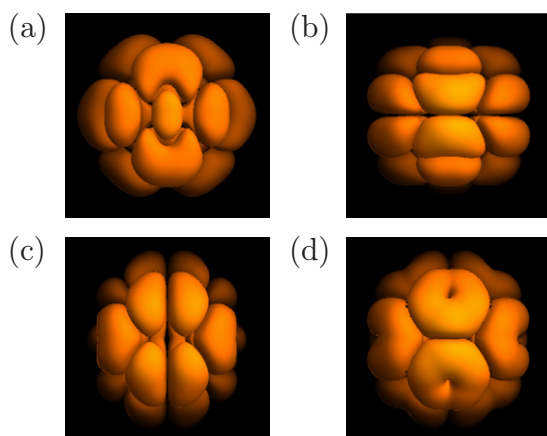
Figure 8. STM simulations of (a) \psi_z^2 , (b) \psi_x^2 , (c) \psi_y^2 and (d) \psi_x^2 + \psi_y^2 orbitals of a double-bond prone C_{60}^- ion.
