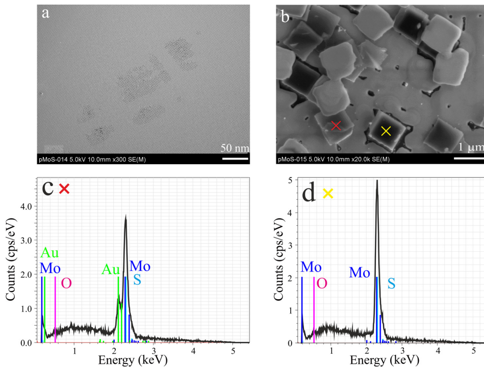
FIG. 7. (Color online) SEM overview and higher resolution image of the stamp surface after printing at large (a) and small scale (b). (c) and (d) EDX spectra taken on top of a decapped pillar (d) and likely a residual of a capping layer (c).
