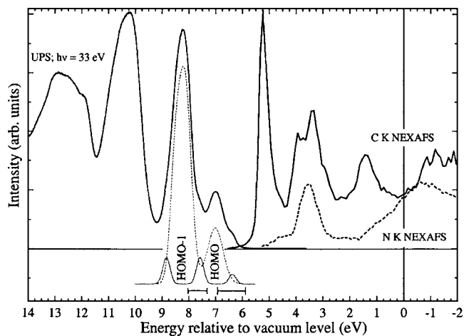
FIG. 1. Combined valence band PES, C K , and N K NEXAFS spectra plotted on a common energy scale, referenced to the vacuum level (Ref. 18). The Gaussian peaks underneath the PES spectrum indicate the HOMO and HOMO-1 (gray, dashed), which are similar to those of C 60 . The other three peaks at 6.37 (HOMO +5 ), 7.58 (HOMO-1 +5 ), and 8.84 eV (HOMO-1 -5 ) indicate peaks with appreciable nitrogen character (gray, solid). The horizontal bars indicate the energy windows used in the constant initial state measurements (see text).
