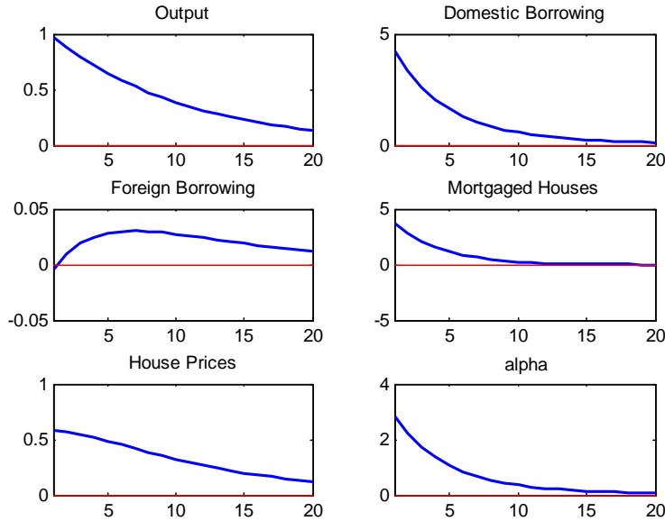
Figure 2: Impulse Responses to a Technology Shock
