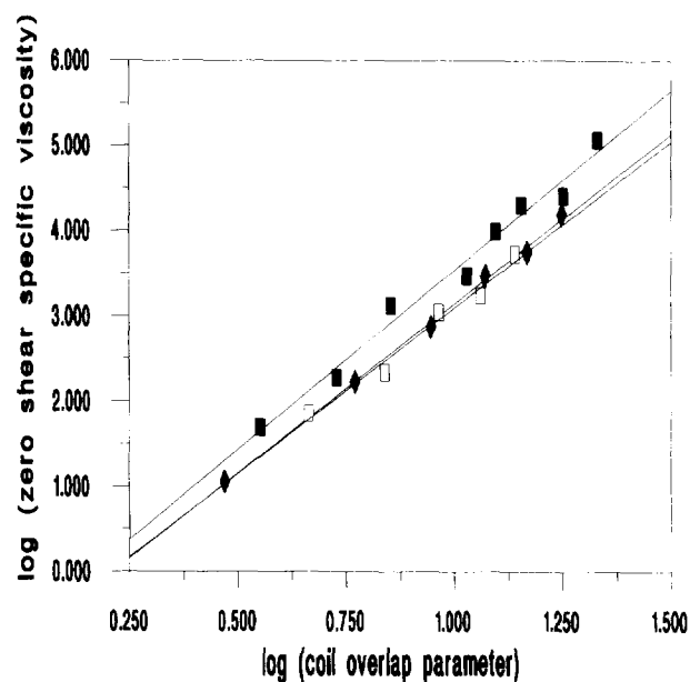
Fig. 4. Double logarithmic plot of zero shear specific viscosity versus the coil overlap parameter [\eta] . The intrinsic viscosity, [\eta] used was that obtained in water. Lines are least squares fits to the data points \blacklozenge : K15M; \square : K8515; \diamond : XU40468.
