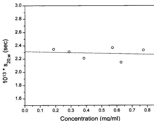
FIGURE 3: Concentration dependence of the sedimentation coefficient, s_{20,w} , for mefp-1 in acetate buffer (pH = 1 = 0.10) at 20 °C.
