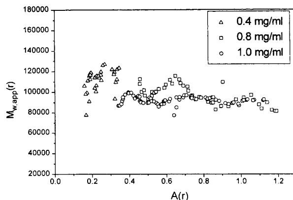
FIGURE 1: Plot of point weight average molecular weights, M_{w,app}(r) , versus local concentration [expressed as absorbance units at 265 nm, A(r) ] at various radial positions r in the ultracentrifuge cell for different loading concentrations (0.4, 0.8, 1.0 mg/mL).
