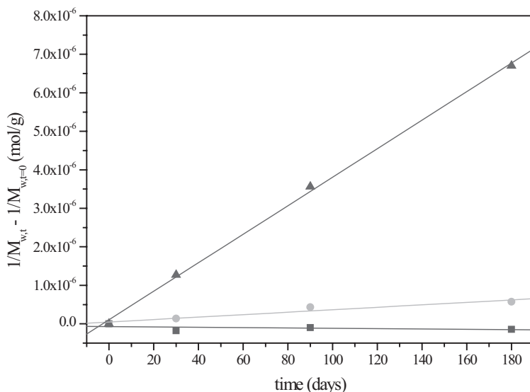
Figure 12. 1 st order kinetic plots of (mol/g) vs. time (days) for pectin of DM ~ 19 %, where closed symbols represent molar masses estimated from viscometry at 4 °C (■), 25 °C (●) and 40 °C (▲) (adapted from Figure 3 in Morris, et al. (2010b)). The kinetic rate constants (day -1 ) are (-0.8 \pm 1.1) \times 10^{-7} , (5.7 \pm 1.1) \times 10^{-7} and (6.7 \pm 0.2) \times 10^{-6} at 4 °C, 25 °C and 40 °C, respectively.
