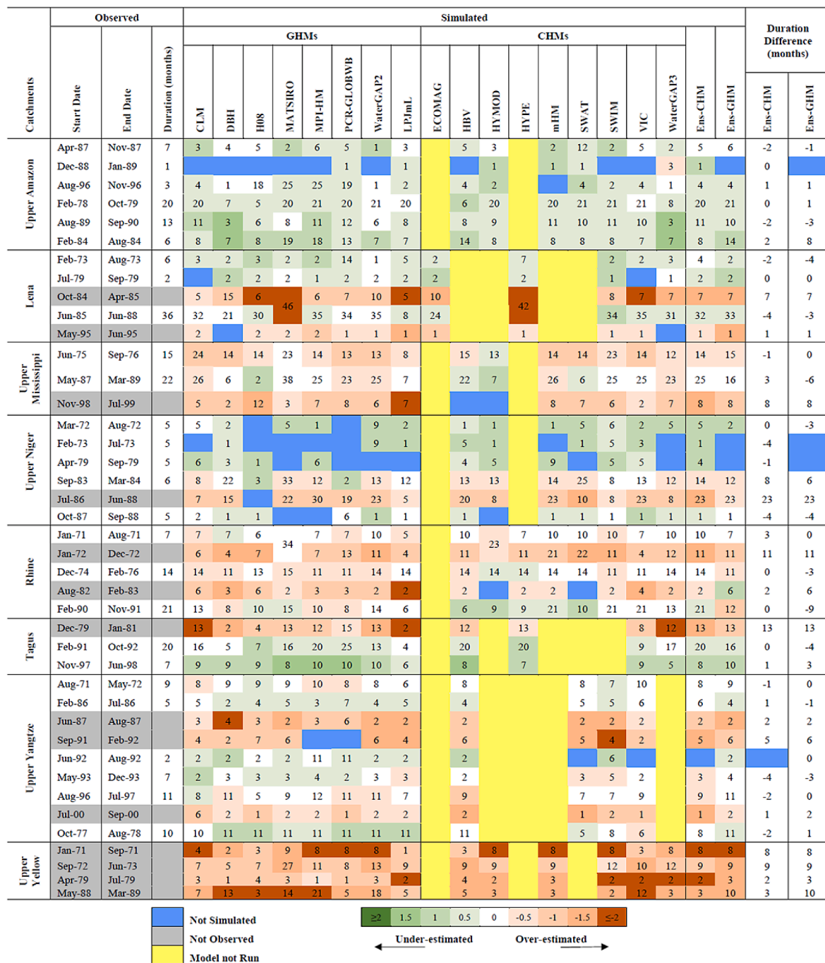
Fig. 2. Observed and simulated extreme SRI drought events ( SRI \leq -2 ). Displayed is each observed drought's start and end date, with the numbers indicating the observed and simulated drought duration in months. Drought events are colour coded based on the difference in simulated and observed drought intensity (from 2 to -2 ), marked from shades of green to brown (under- and over-estimated respectively). Blue cells are observed droughts not present in simulated records. Grey cells are simulated droughts (either by Ens-CHM or Ens-GHM or both) not present in the observed record. Yellow cells denote that the particular model was not run for the specific catchment.
