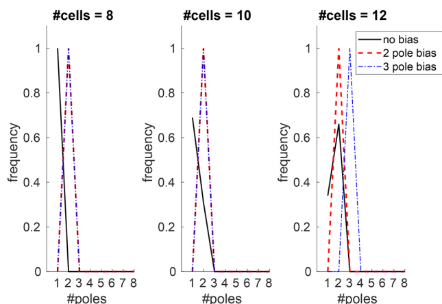
Fig. 6. Heterogeneous input of auxin can establish robust patterns that might otherwise be unstable. Pole frequency plots for differently sized templates based on 100 simulations. All simulations have stochastic fluctuations in initial auxin according to a normal distribution (see supplementary Materials and methods for details). The black lines represent simulations with uniform auxin production (as in Figs 4 and 5). Red dashed lines represent a persistent bias in auxin production in two opposite cells; blue dot-dashed lines represent a temporary bias in auxin input in three approximately equally spaced cells (owing to the restrictions from using integer values).
