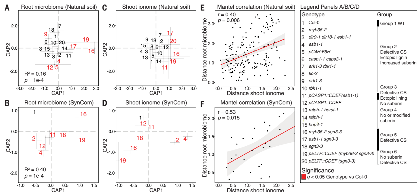
Fig. 1. Plants with modified root diffusion barriers assemble a distinct microbiome. (A and B) CAP analysis of root microbiome composition showing the projected microbiome assembly of the root diffusion barrier genotypes (numbers) in plants grown in (A) natural soil and (B) agar plates inoculated with a bacterial synthetic community (SynCom). (C and D) CAP analysis of shoot mineral nutrient composition (ionome) showing the projected ionomic profiles of
