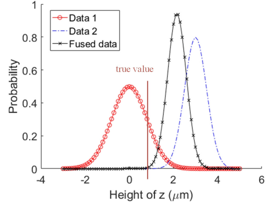
(b) Measurement with large systematic error but small random error, fused with measurement with small systematic error and large random error, M1 < Tv < M2
