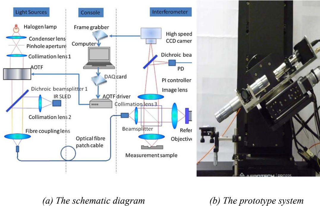
Figure 2.49 The wavelength scanning interferometry system (Jiang, 2011)
