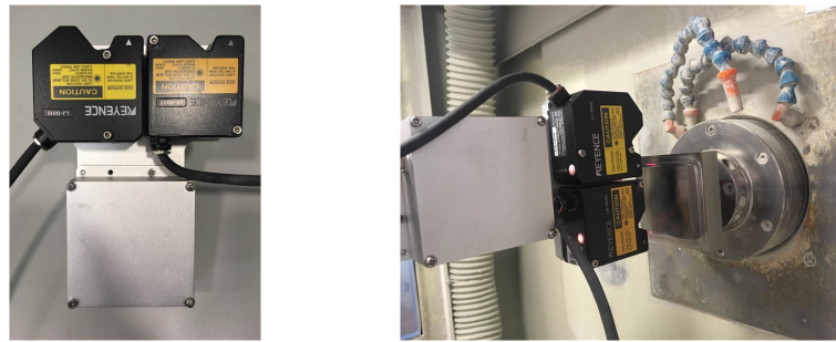
(a) Assembled sensor module (b) Installation in the machine tool
