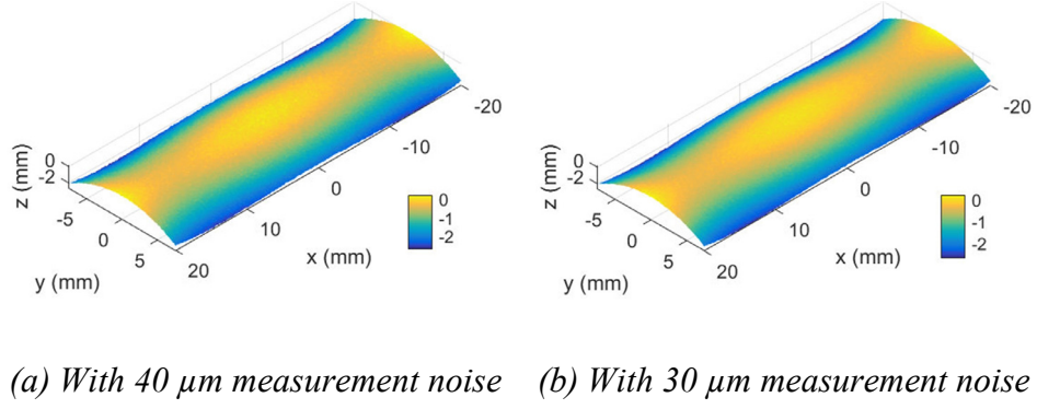
Figure 4.10 Simulated measurement results of the designed f -theta lens surface
