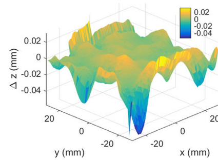
(c) Deviation from reference data
