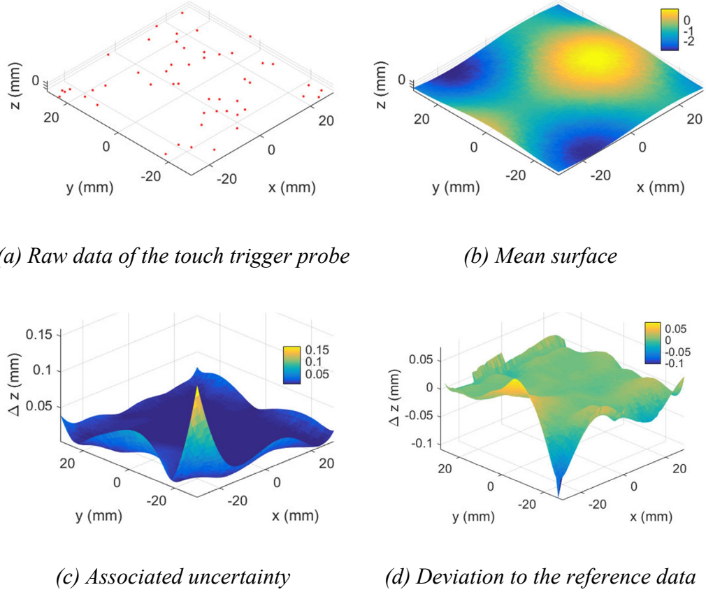
Figure 4.20 Measurement data of touch trigger probe and Gaussian process result
