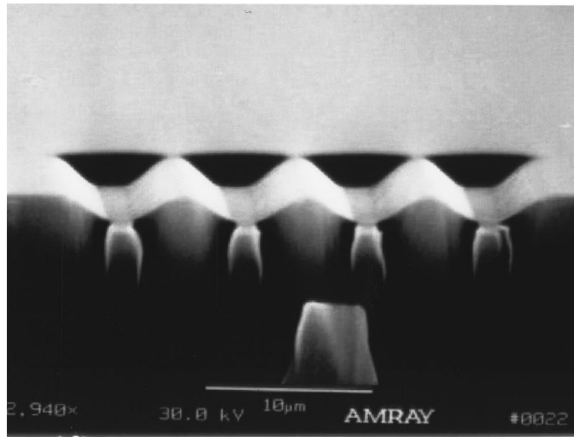
Figure 2.15 SEM image of the sinusoidal wave machined by focused ion-beam milling (Vasile et al., 1999)
