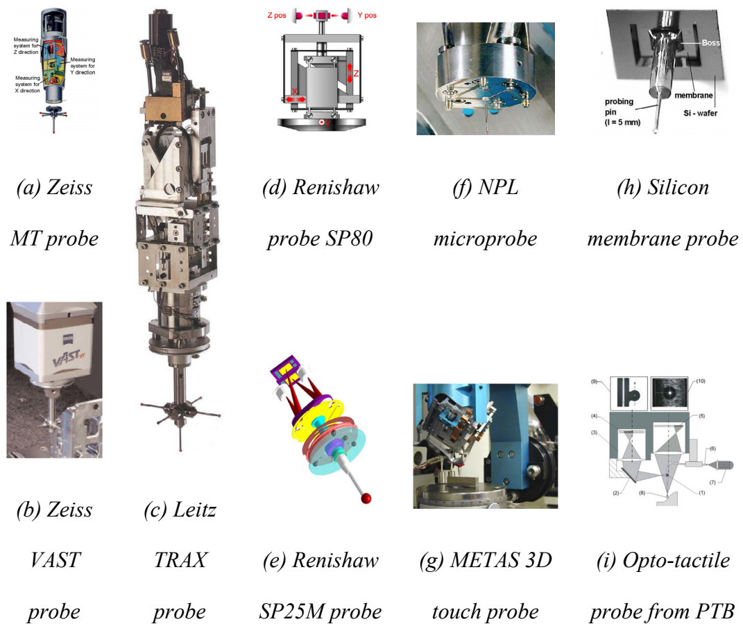
Figure 2.27 Varies kinds of probing systems (Weckenmann et al., 2004)
