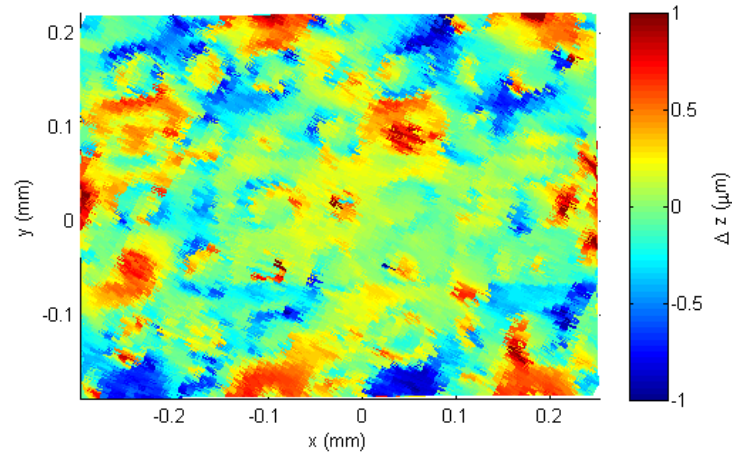
Figure 3.14 Proposed stitching error comparing with a single shot measurement
