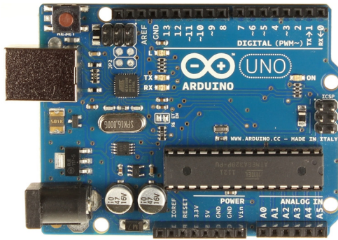
(c) Arduino Uno board
