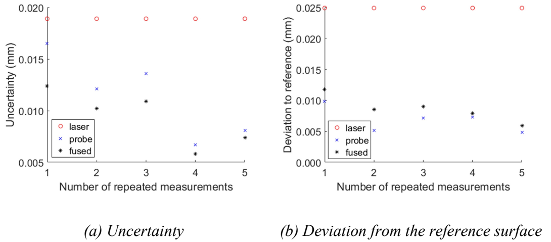
Figure 4.27 Repeated measurement result
