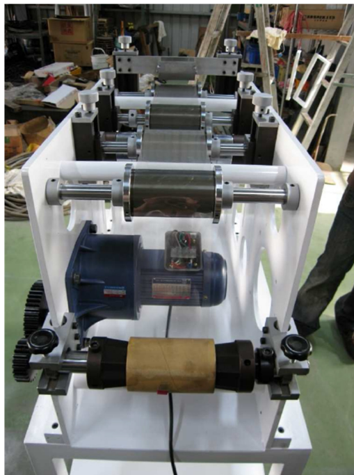
(a) The roll-to-roll equipment
