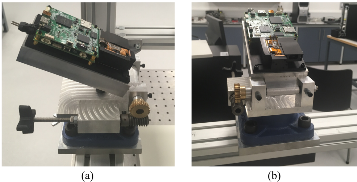
Figure. 4.23 Multi-view fringe projection projector mount, designed to provide adjustability in the pitch and yaw axes of rotation. (a) Side on view and (b) front on view.
