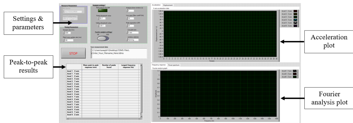
Figure. 6.5 Front panel LabVIEW display of the multi-accelerometer host VI, which allows the user to control the system and view the measurement results.
