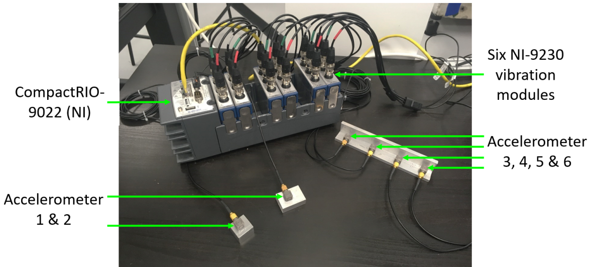
Figure. 6.1 The developed multi-accelerometer live monitoring system, which includes six triaxial IEPE accelerometers, a CompactRIO-9022 controller, with an eight module slot chassis attached and six NI-9230 vibration and sound modules integrated.
