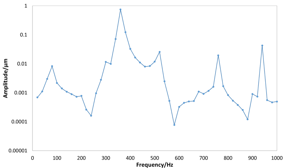
Figure. 4.19 ANSYS simulation results for the frequency response of the full frame assembly, which shows the largest response and natural frequency of the system is at 360 Hz.
