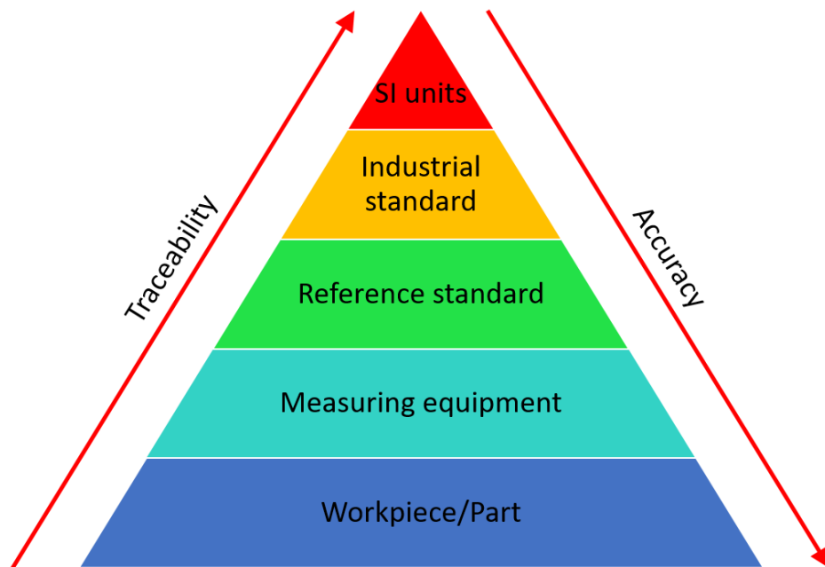
Figure. 1.1 The traceability pyramid. In order to ensure traceability is transferred between each level by calibration, and creates a traceable unbroken chain from the measured part to the definition of the SI unit.
