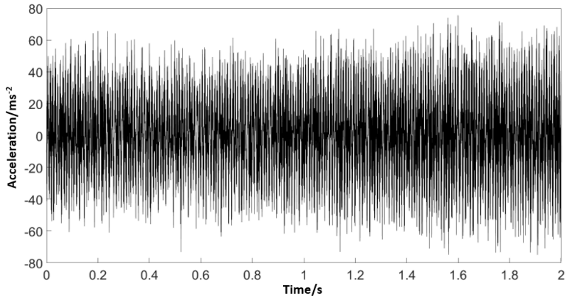
Figure. 3.4 An exemplar vibration dataset collected using an accelerometer mounted on a lathe during the cutting process.
