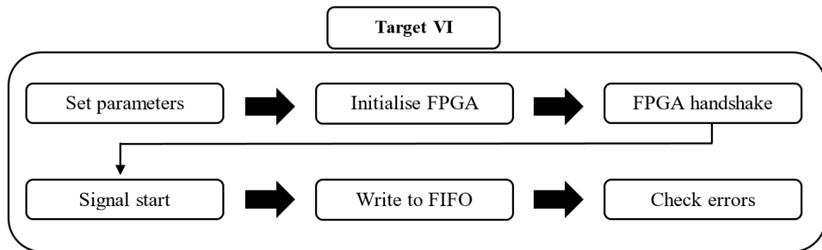
Figure. 6.2 Top-level programme function flowchart of the designed target VI, which is compiled onboard the cRIO, to collect and stream the accelerometer data to the host VI.
