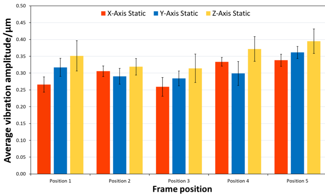
Figure. 5.15 Full frame three axis characterisation results in 5 key positions with no excitation applied to the frame.
