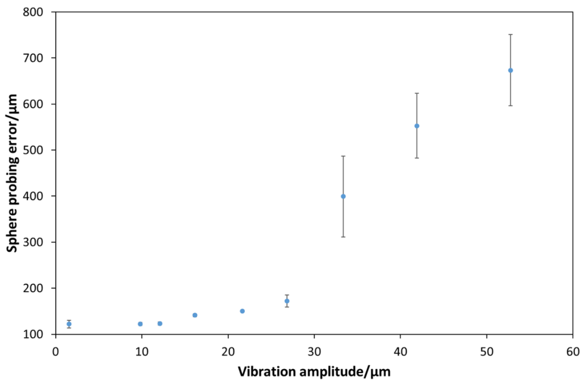
Figure. 7.3 A plot of increasing the amplitude of vibration in the x -axis against the sphere probing error (mean between the positive and negative) of a fitted sphere to the ball of the ball bar fixture on the AM artefact, shows how fringe projection measurements deteriorate on complex features as the vibration levels increase.
