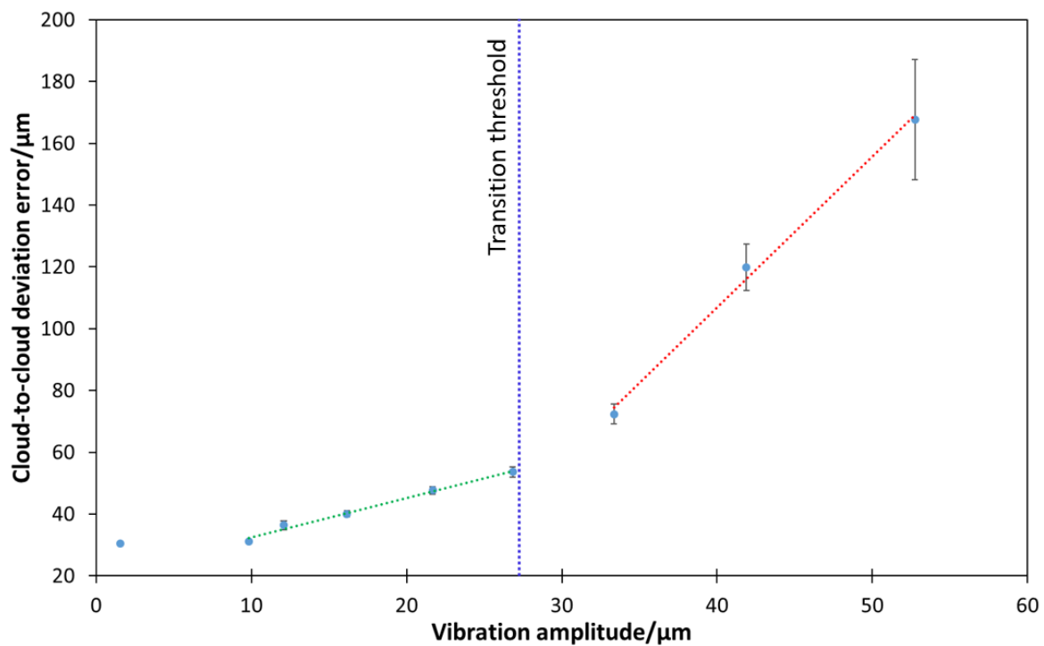
Figure. 7.2 A plot of increasing the amplitude of vibration in the x -axis against the mean cloud-to-cloud measurement error showing a sharp increase in the linear trend between the red and green dashed lines, which is due to the significant measurement errors seen around the edges of the complex features on the artefact. The blue dashed line shows the defined acceptable measurement threshold at the point the trends change.
