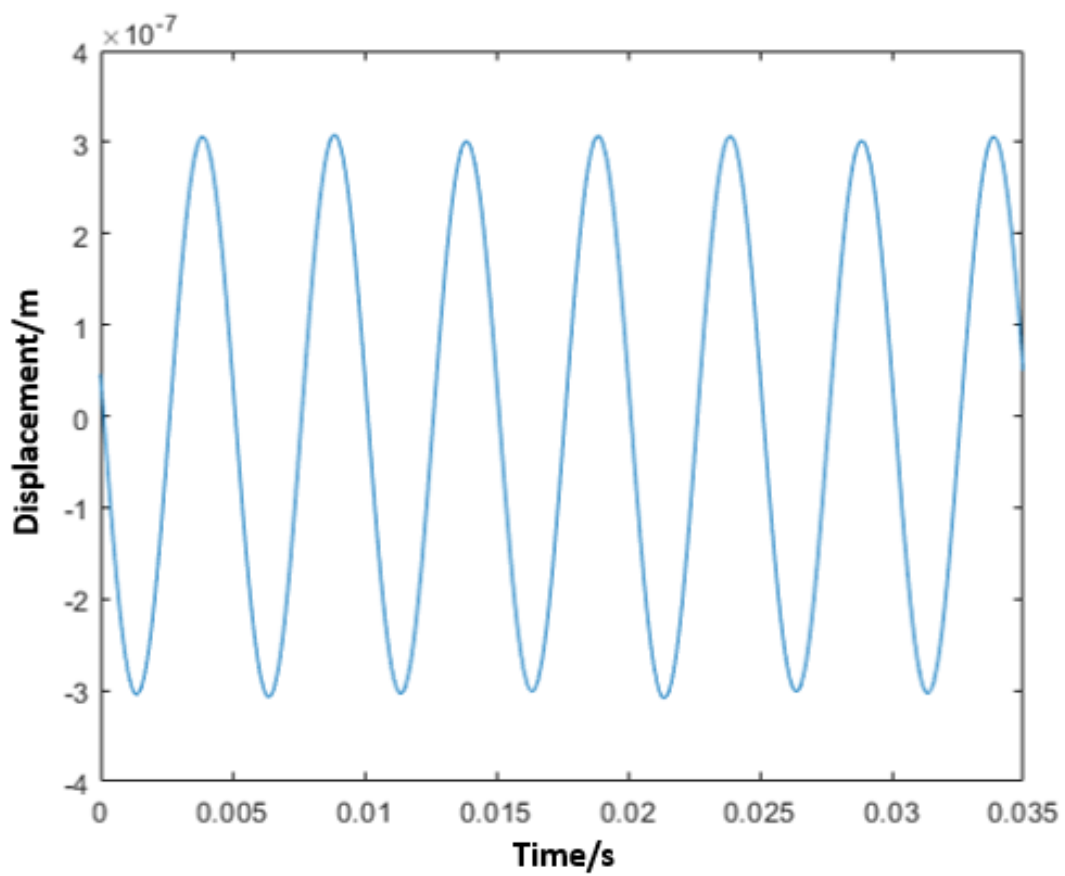
Figure. 5.12 The displacement data obtained using the omega arithmetic method to convert the acceleration data with a Butterworth filter applied.
