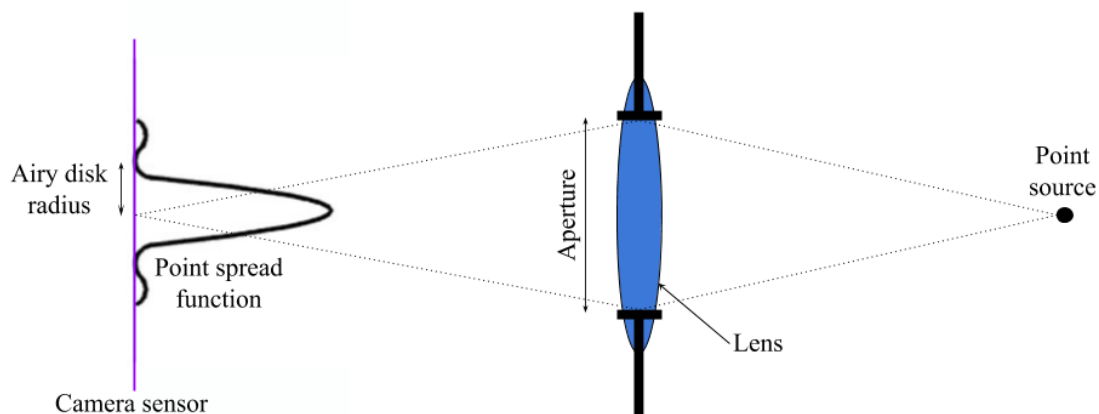
Figure. 2.7 Point spread function produced by a point source passing through a simple optical system consisting of a lens and circular aperture.
