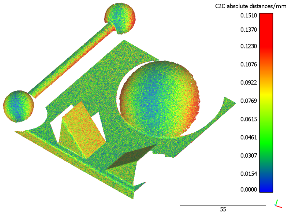
Figure. 7.5 Heat map of the cloud-to-cloud error analysis for 0.25 V vibration input of the shaker in the x -axis, showing the large measurement errors around the edges of the complex shapes on the AM artefact, i.e. the large sphere due to the triangulation errors caused by vibration.
