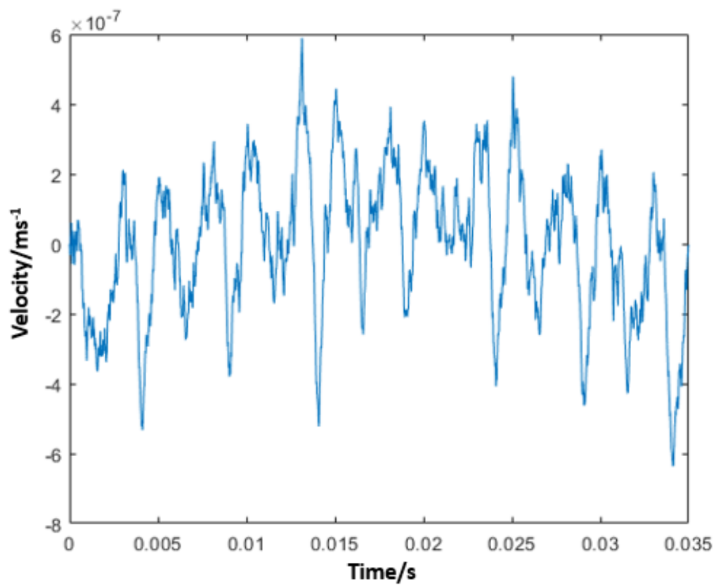
Figure. 5.9 The velocity data obtained using the integration method and the acceleration data with the bias removed and the Butterworth filter applied.
