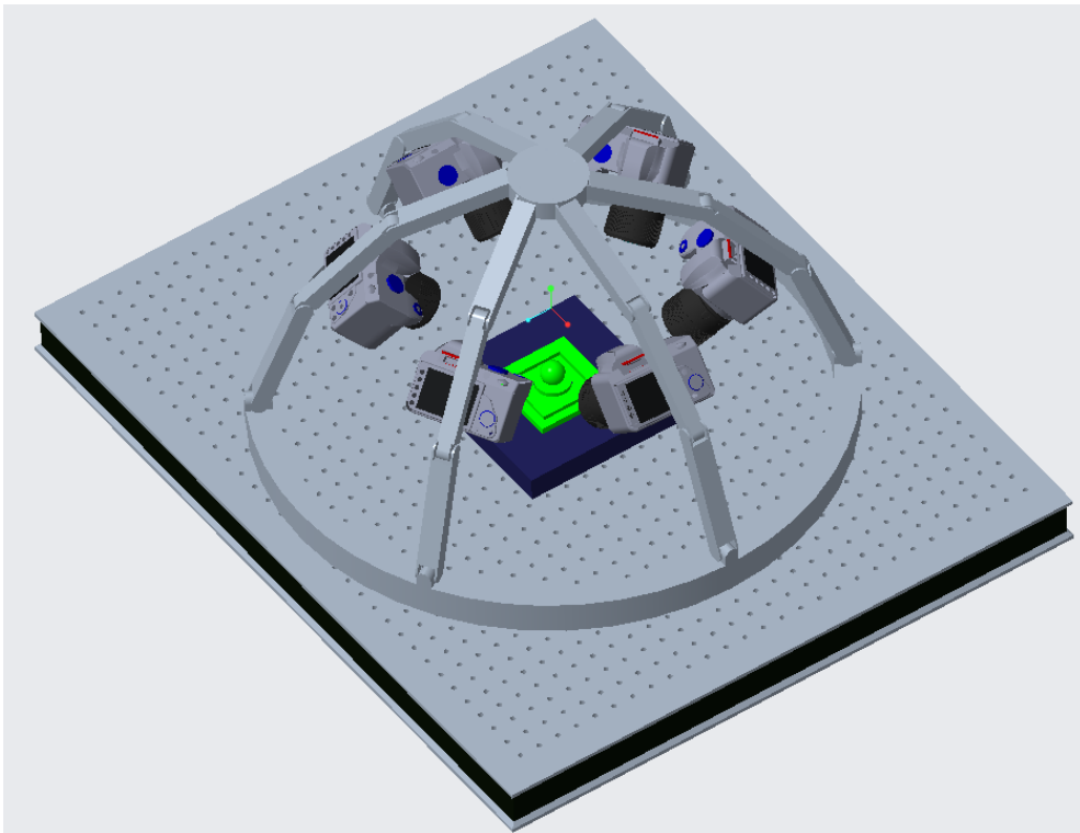
Figure. 4.13 CAD representation of the fifth concept ('linkage cage') proposed as a design solution for the multi-view fringe projection system.
