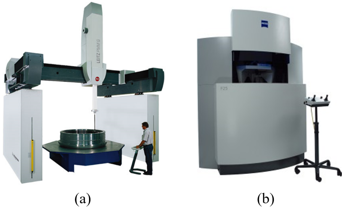
Figure. 2.1 Example of an (a) large-scale CMM from Leitz and (b) a small-scale CMM from Zeiss
