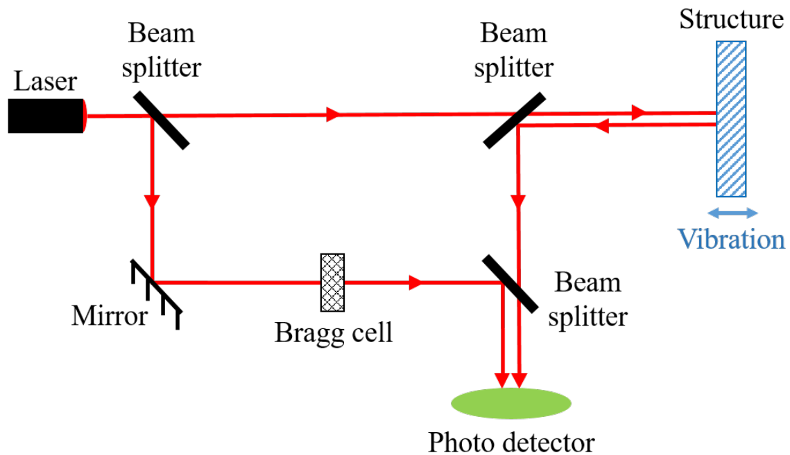
Figure. 5.3 Schematic diagram depicting the key elements of a laser vibrometer.
