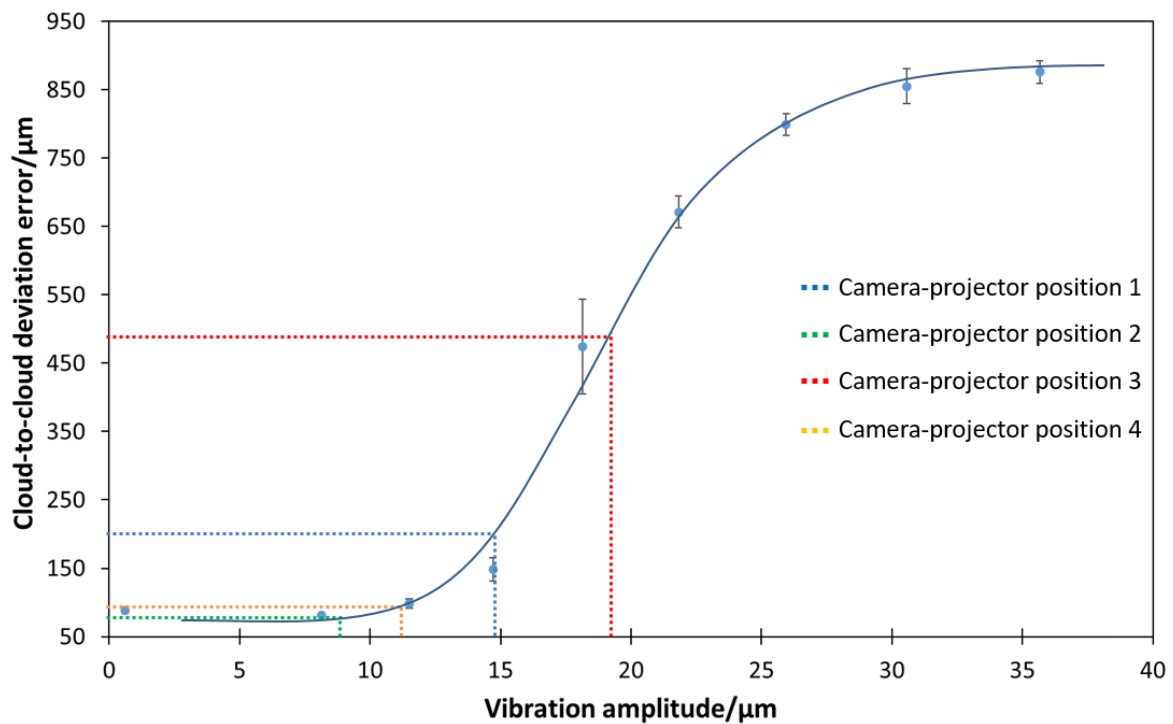
Figure. 7.19 Demonstrating the importance of condition monitoring in measurement systems, by showing an example of the different measurement errors (cloud-to-cloud) that could be experienced by each camera-projector pair in the multi-view fringe projection system due to the varying vibrations seen across the measurement frame.
