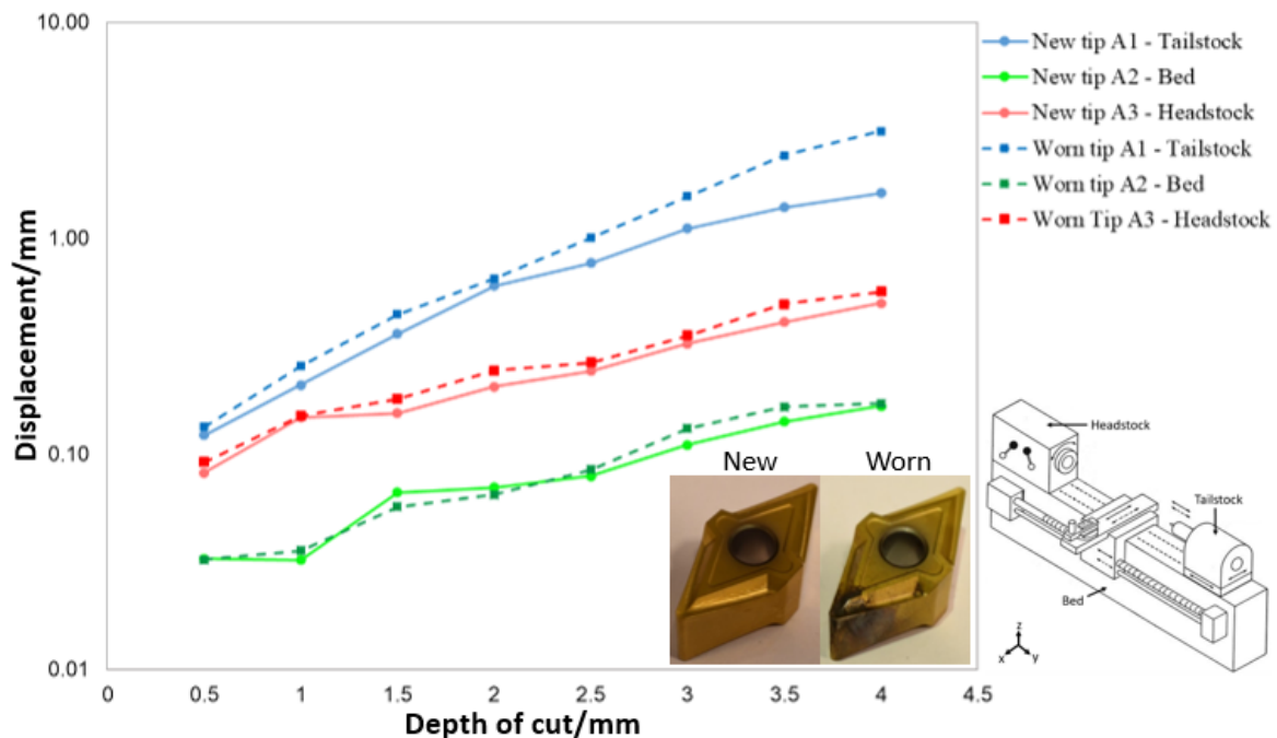
Figure. 6.14 Vibration results in the y-axis for the effect of increasing depth of cut and tool wear, showing the vibration increases that can be measured as the cutting tip progressively wears to predict tool failure.
