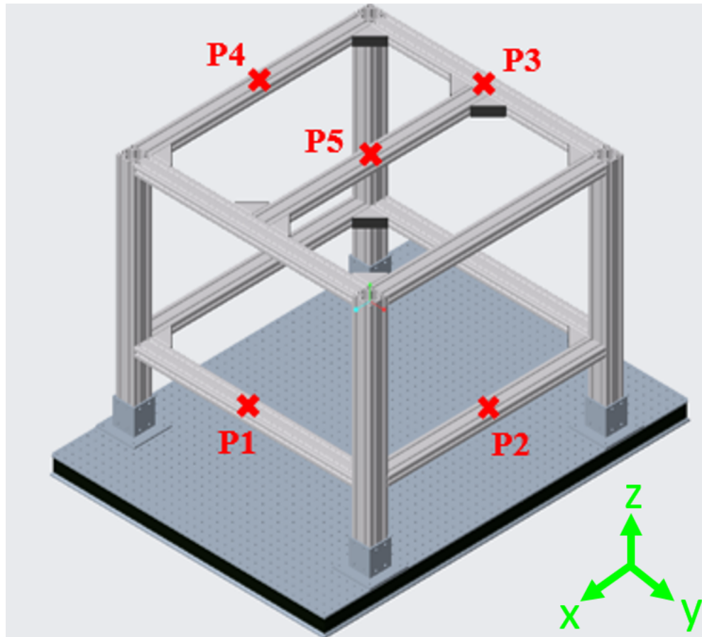
Figure. 5.14 Key locations identified around the multi-view frame to study the vibrational response of the system in both a non-excited and camera excited state.
