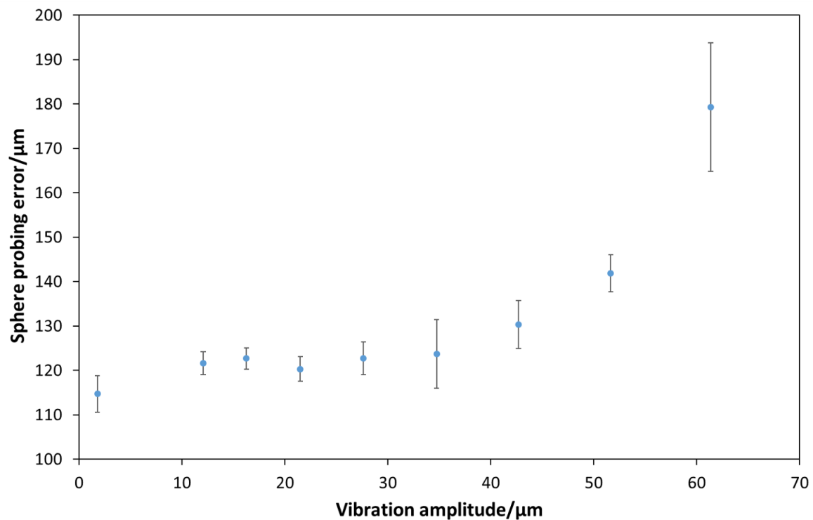
Figure. 7.7 A plot of increasing the amplitude of vibration in the y-axis against the sphere probing error (mean between the positive and negative) of a fitted sphere to the ball of the ball bar fixture on the AM artefact, shows how fringe projection measurement deteriorate on complex features as the vibration levels increase.
