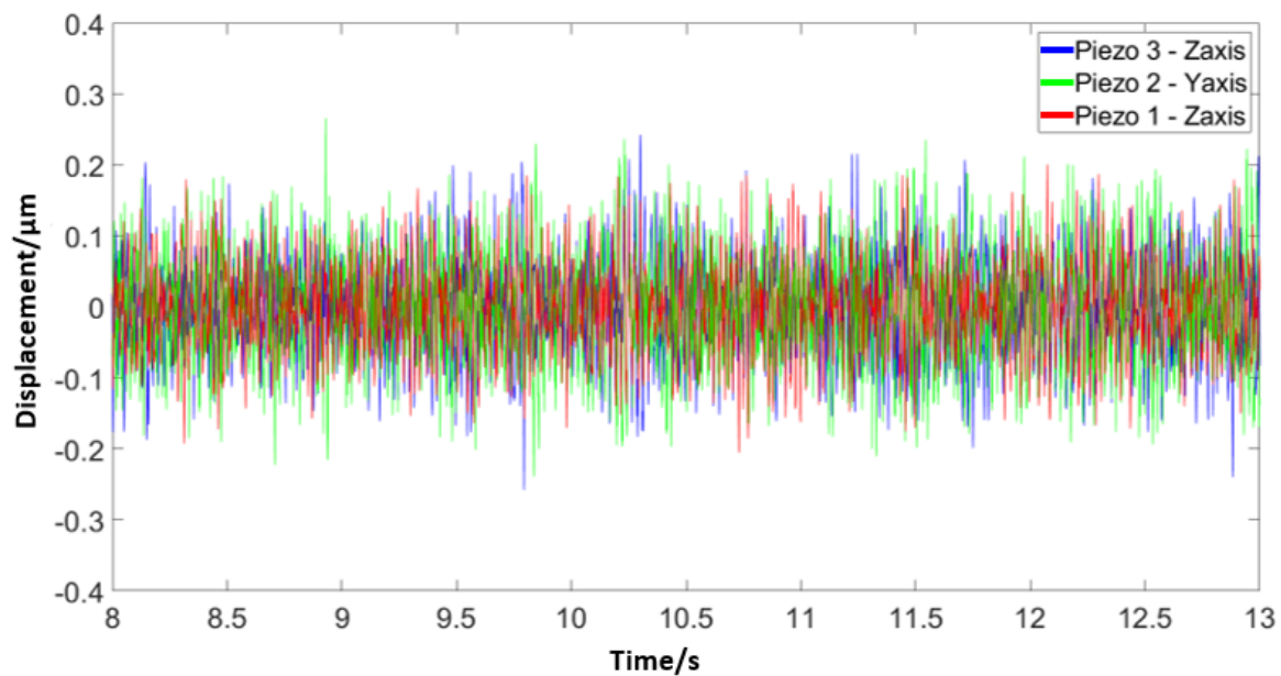
Figure. 6.7 Displacement results for the three channels that have been identified to have the largest average responses in the system within the time window analysed, which was 5 seconds in the example shown.
