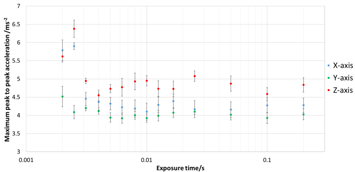
Figure. 4.17 Camera excitation characterisation results, the averaged peak-to-peak response in each of the x , y and z axes, is plotted against log of changing exposure time, and shows that the response of the camera is increased at smaller exposure times but the exposure time negligible effect at the longer exposure times.
