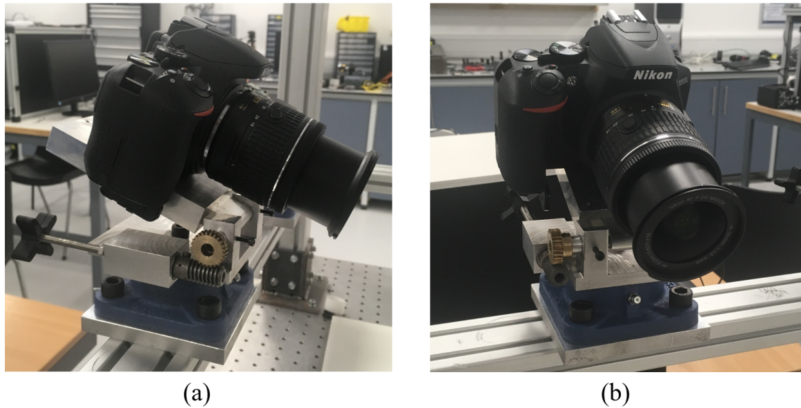
Figure. 4.21 Multi-view fringe projection camera mount, designed to provide adjustability in the pitch and yaw axes of rotation. (a) Side on view and (b) front on view.
