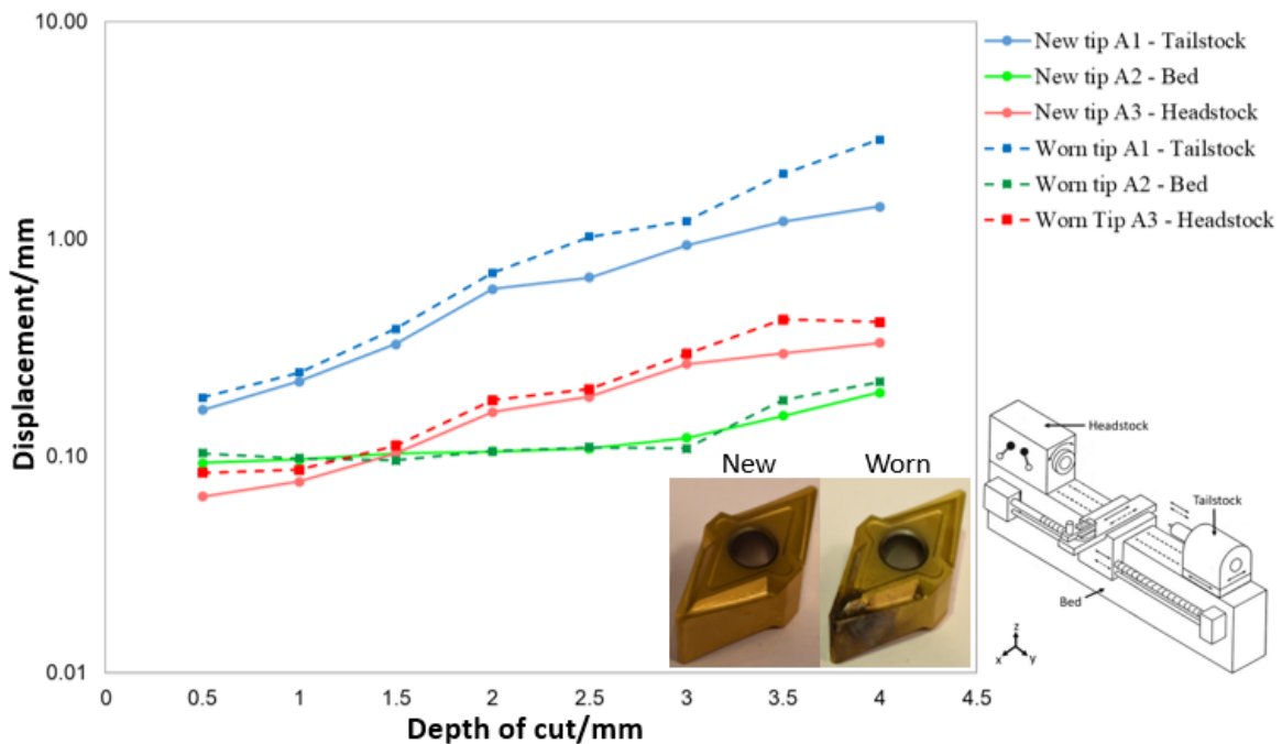
Figure. 6.13 Vibration results in the x -axis for the effect of increasing depth of cut and tool wear, showing the vibration increases that can be measured as the cutting tip progressively wears to predict tool failure.
