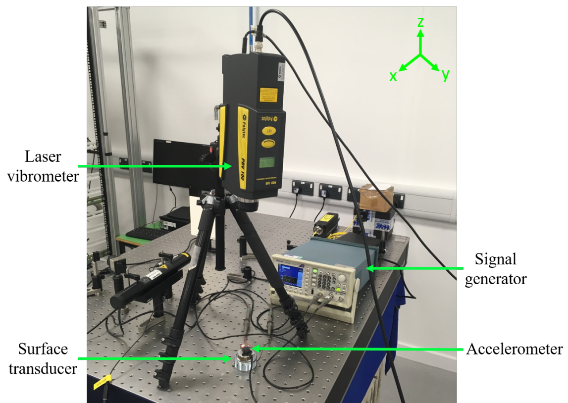
Figure. 5.4 The experimental setup used to investigate the proposed acceleration to velocity/displacement conversion methods, using a piezoelectric accelerometer, digital oscilloscope and surface transducer. A laser vibrometer was used to verify the behaviour of the surface transducer and the measured accelerometer data.
