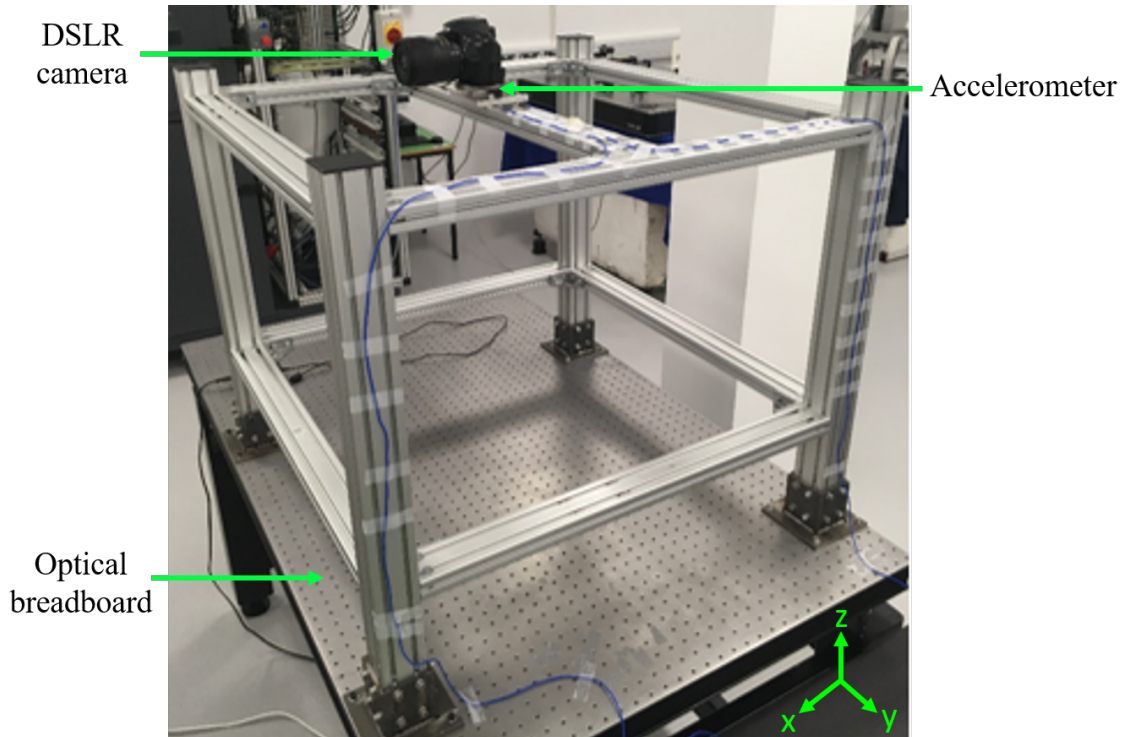
Figure. 4.16 Experimental setup to characterise the excitation that the DSLR camera inputs into the metrology frame, using a triaxial accelerometer to measure the acceleration when capturing images.
