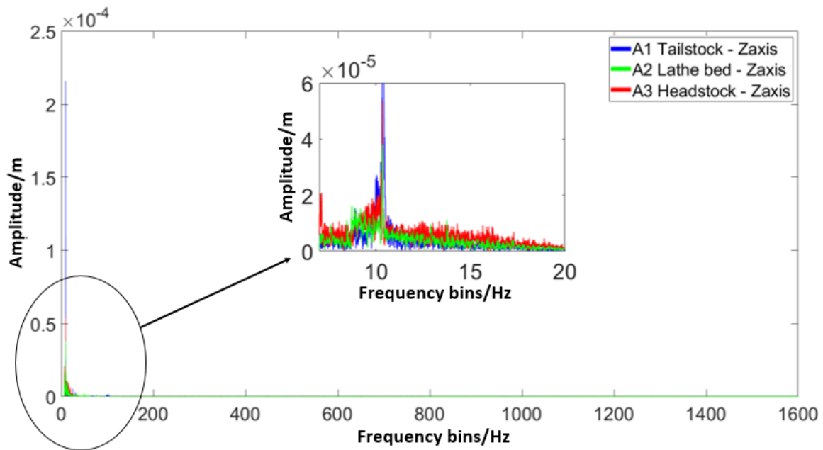
Figure. 6.12 Example frequency response analysis plot of the measured vibration dataset collected whilst performing a 2.0 mm depth of cut on a CNC lathe using a new cutting tip, showing the largest response at 10 Hz, which matches the frequency of the spindle.
