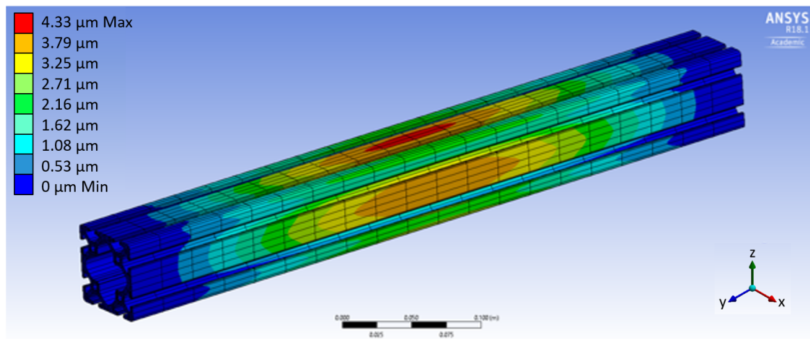
Figure. 4.14 Heat map of the maximum deformation on a 60 mm \times 60 mm aluminium extrusion profile showing how the excitation force applied to the middle of the strut propagates around the part.
