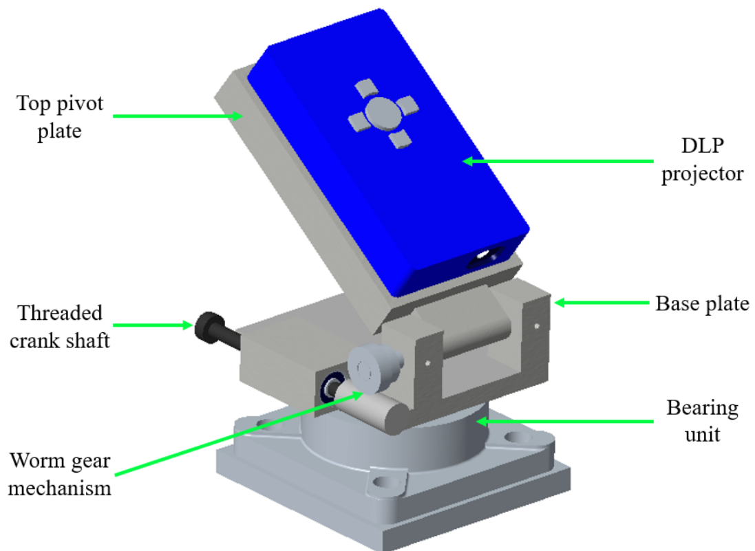
Figure. 4.22 CAD schematic of the projector mount design that was used in the multi-view fringe projection system.
