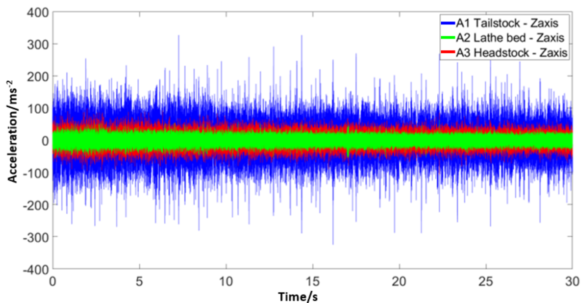
Figure. 6.11 Example measured vibration dataset in the z -axis, collected whilst performing a 2.0 mm depth of cut on a CNC lathe using a new cutting tip.
