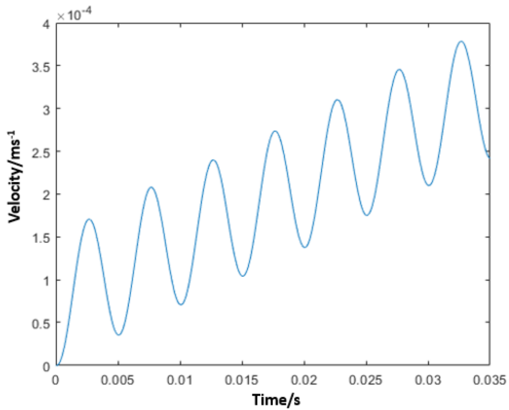
Figure. 5.6 The velocity dataset obtained using the raw measured z -axis acceleration data of a 200 Hz sinusoidal signal and the integration method to convert to velocity.
