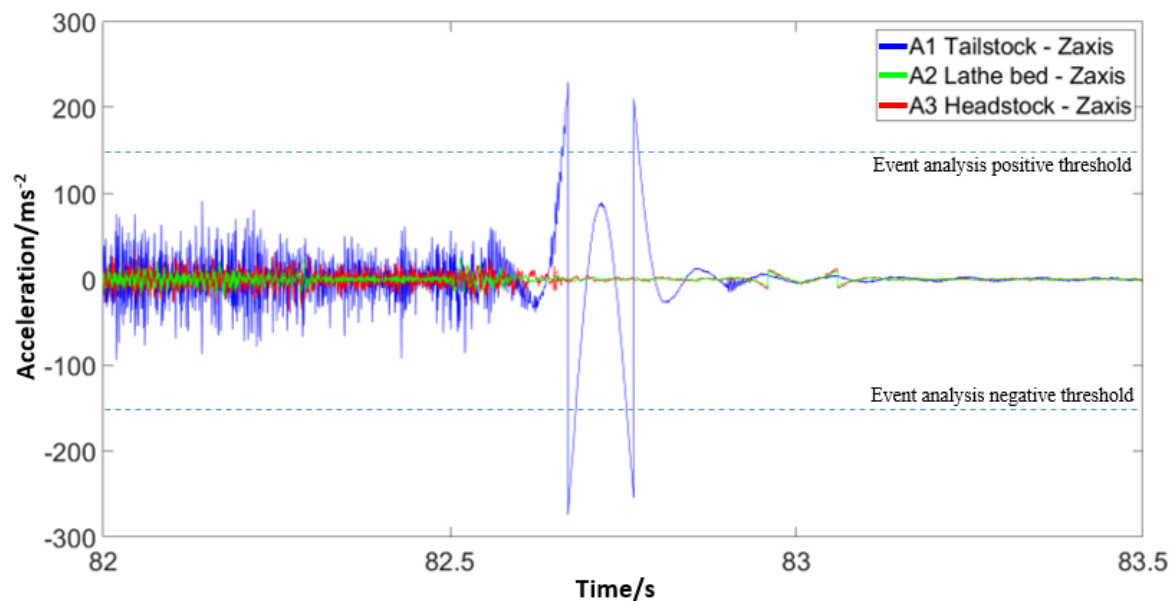
Figure. 6.16 Example of an ‘event’ identified by the event analysis tool, as the measured signal exceeds the user defined thresholds (dashed lines). In this example, the ‘event’ is as a result of the brake being applied to stop the spindle after the cutting process has finished.
