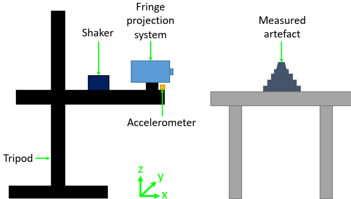
Figure. 7.1 Schema of the experimental setup using the GOM ATOS Core 300, a triaxial accelerometer and a Smart Shaker K2007E01 to investigate the sensitivity of a commercial fringe projection system to vibration.
