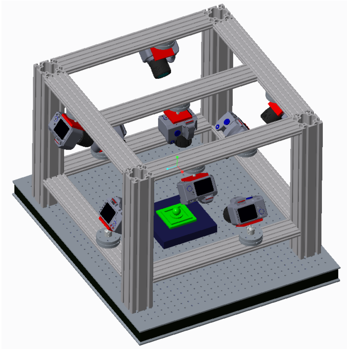
Figure. 4.15 CAD model of the final multi-view frame design, using 60 mm \times 60 mm aluminium profile for the vertical posts, and 60 mm \times 30 mm aluminium extrusion for the horizontal beams, based on the results of the FEA simulations.
