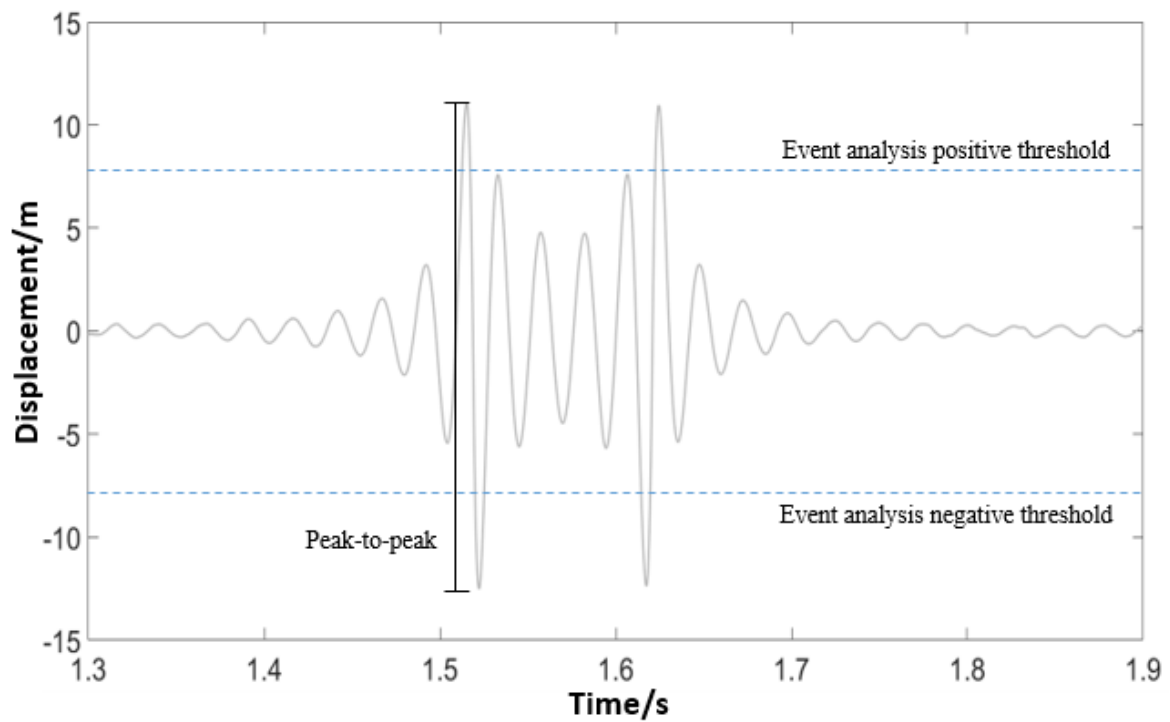
Figure. 6.4 The event analysis plot to investigate the dynamic behaviour around the area of interest, which is identified by the peak above the user defined threshold (dashed line), with the peak-to-peak analysis also illustrated.
