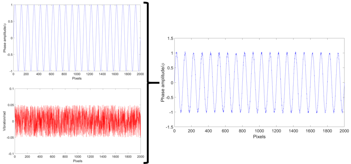
Figure. 4.1 An example dataset created using the simulation method of combining the ideal sinusoidal phase shifting pattern with a normalised pseudo-random noise signal to create simulated noisy fringe projection images.
