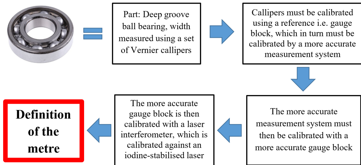
Figure. 1.2 Practical example of the traceability chain applied to a length measurement of the width of a ball bearing part.
