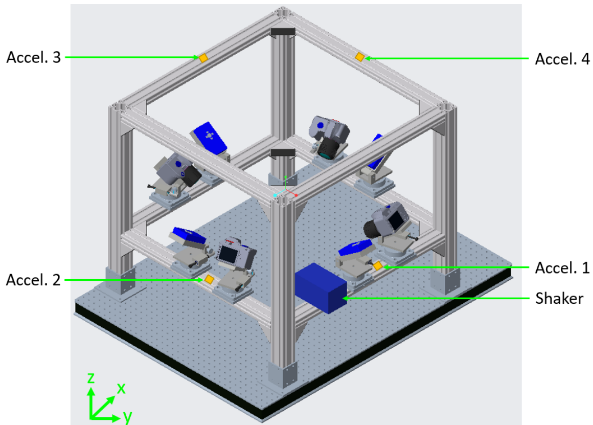
Figure. 7.10 Schema of the experimental setup using the developed multi-view fringe projection system, four triaxial accelerometers and a Smart Shaker K2007E01 to benchmark the system and investigate the measurement sensitivity to vibration, as well as demonstrate the use of multi-point condition monitoring.
