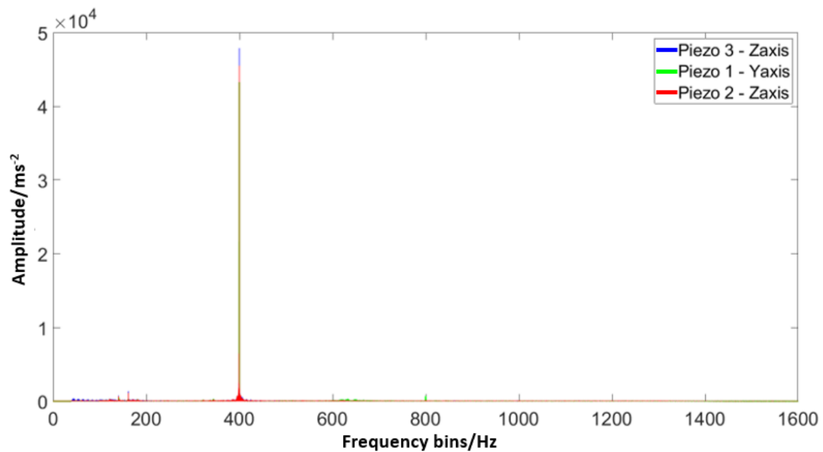
Figure. 6.8 Frequency responses of the three channels identified to have the largest average responses in the system within the time window analysed, which was 5 seconds in the example and shows a dominant excitation input with a frequency of 400 Hz.
