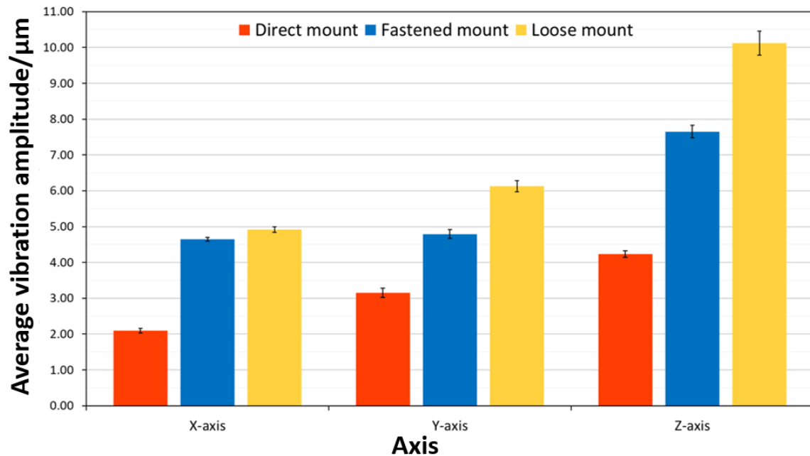
Figure. 5.19 Average characterisation results using a triaxial accelerometer to compare the excitation of the different camera and projector mounts used in the multi-view fringe projection setup, as well as assess the ability of the characterisation method to identify a mechanical fault in the system I.E. the mounts not being fastened properly.
