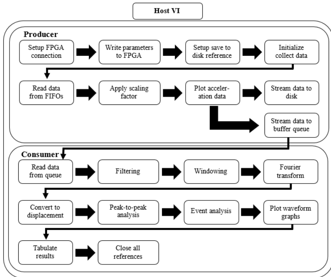
Figure. 6.3 Top-level programme function flowchart of the designed host VI which is executed on the main computer and communicates and reads the accelerometer data from the target VI on the cRIO. The Host VI uses the producer-consumer architecture to read and process data efficiently.
