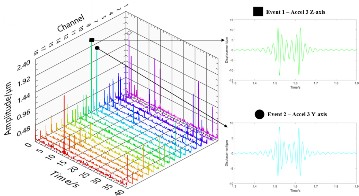
Figure. 6.9 3D stacked ribbon plot of the displacement envelope results for all 18 measurement signals ( x , y and z axes for each accelerometer) with the key events that are identified to be of interest and so further analysed.
