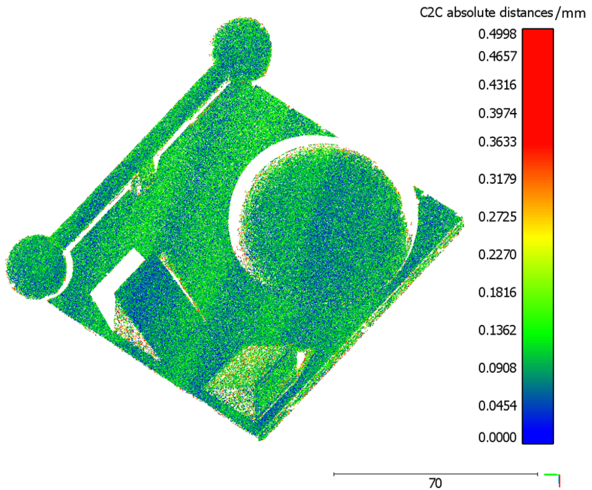
Figure. 7.13 Heat map of the cloud-to-cloud error analysis for 0 V (baseline) vibration input of the shaker in the x -axis, showing the structured modulation errors across the measurement artefact.
