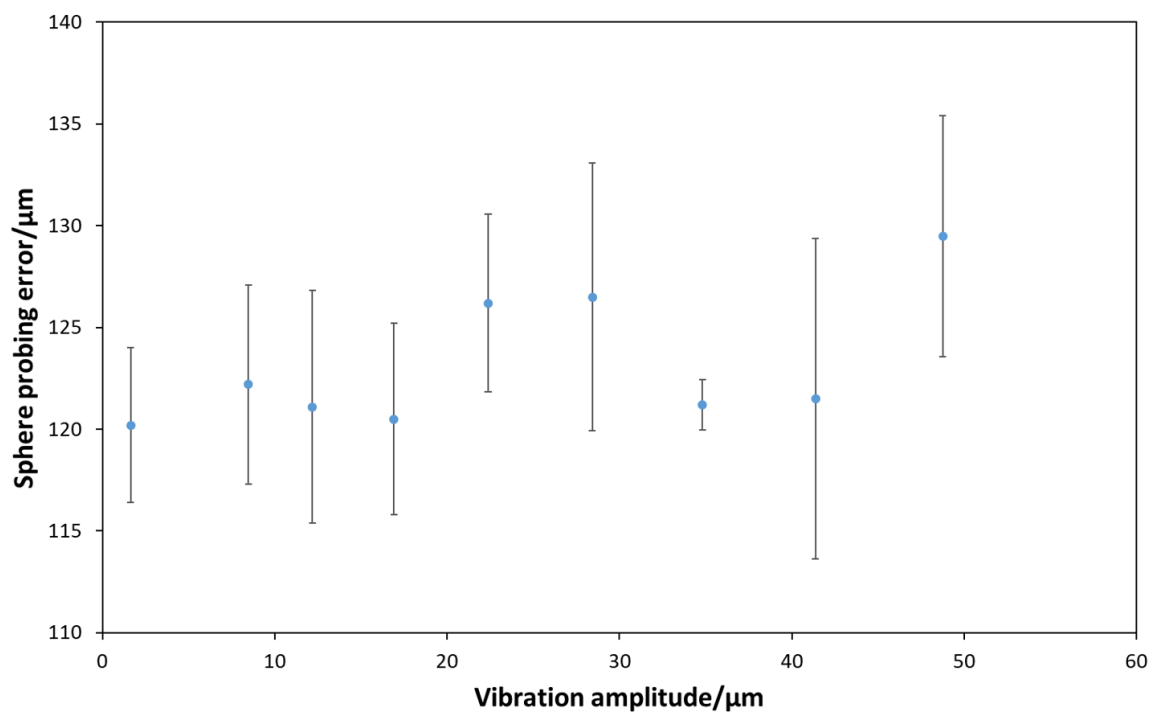
Figure. 7.9 A plot of increasing the amplitude of vibration in the z -axis against the sphere probing error (mean between the positive and negative) of a fitted sphere to the ball of the ball bar fixture on the AM artefact, shows the trend of the sphere probing errors in the z does not match the increasing measurement error trend as it does in the x and y axes.
