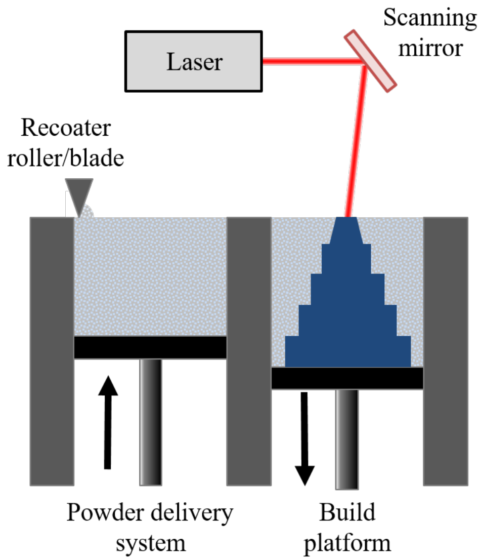
Figure. 3.1 Schematic diagram depicting the process used for additive manufacturing powder bed fusion technologies.
