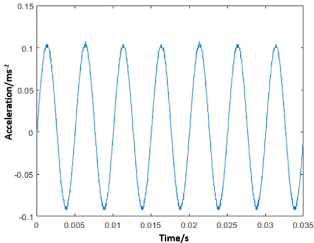
Figure. 5.5 Discrete sample dataset of the raw z -axis acceleration data measured using the piezoelectric accelerometer mounted on the surface transducer generating a 200 Hz sinusoidal signal.
