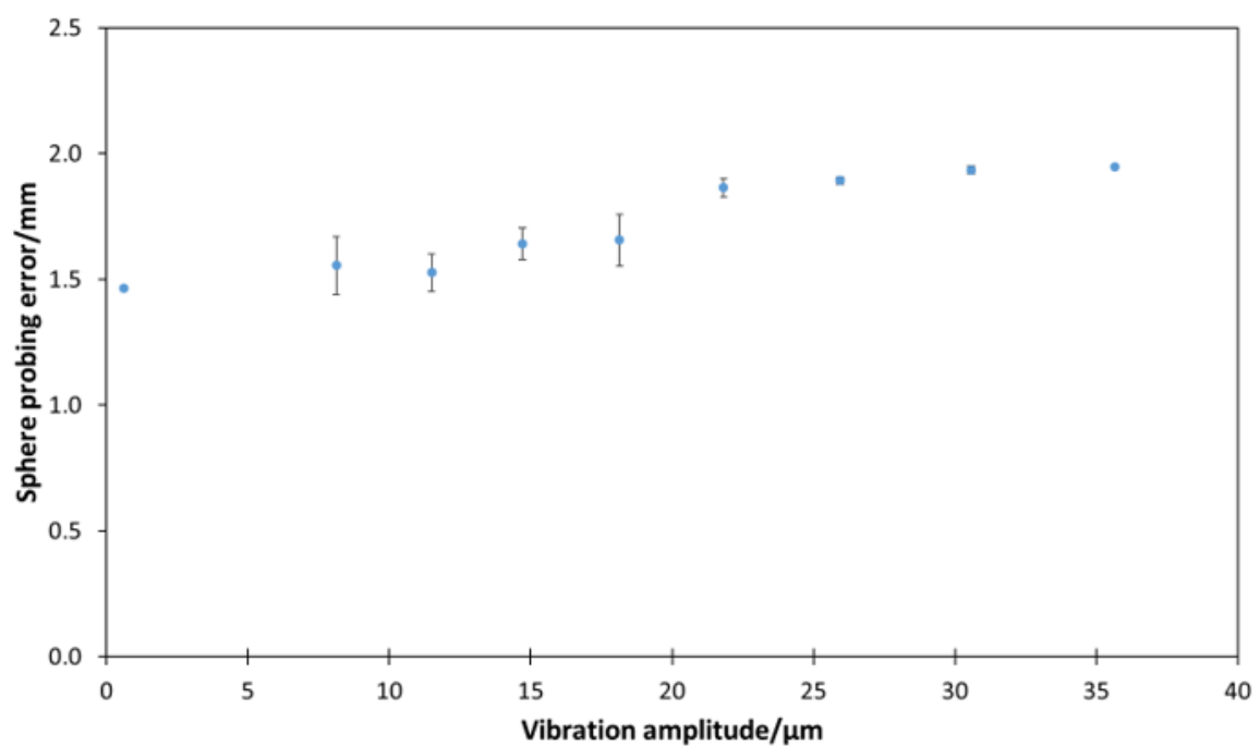
Figure. 7.18 A plot of increasing the amplitude of vibration in the z -axis against the sphere probing error (mean between the positive and negative) of a fitted sphere to the ball of the ball bar fixture on the AM artefact, shows the sphere probing error trend does not match the increasing measurement error.
