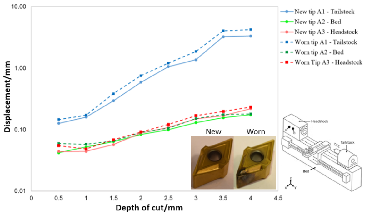
Figure. 6.15 Vibration results in the z-axis for the effect of increasing depth of cut and tool wear, showing the vibration increases that can be measured as the cutting tip progressively wears to predict tool failure.
