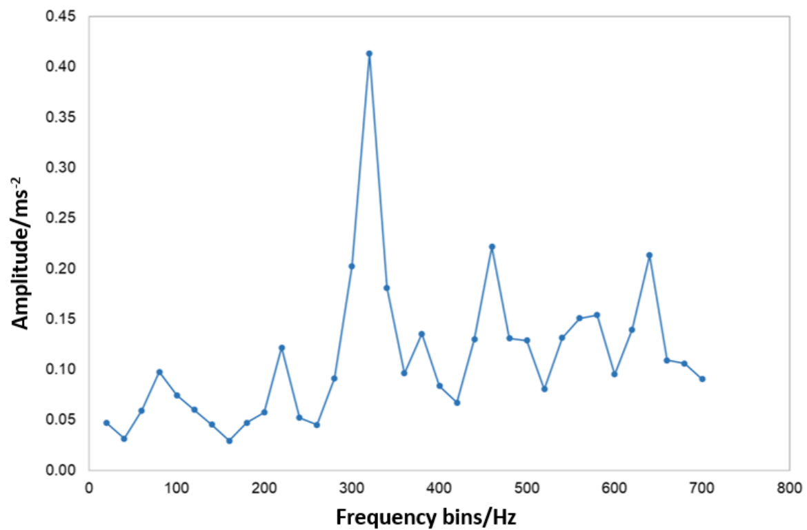
Figure. 5.13 Frequency response experiment on the full frame, applying an excitation in the z -axis with the frequency varied from 20 Hz to 700 Hz, in steps of 20 Hz to study the natural frequency of the frame, which is at \sim 320 Hz.
