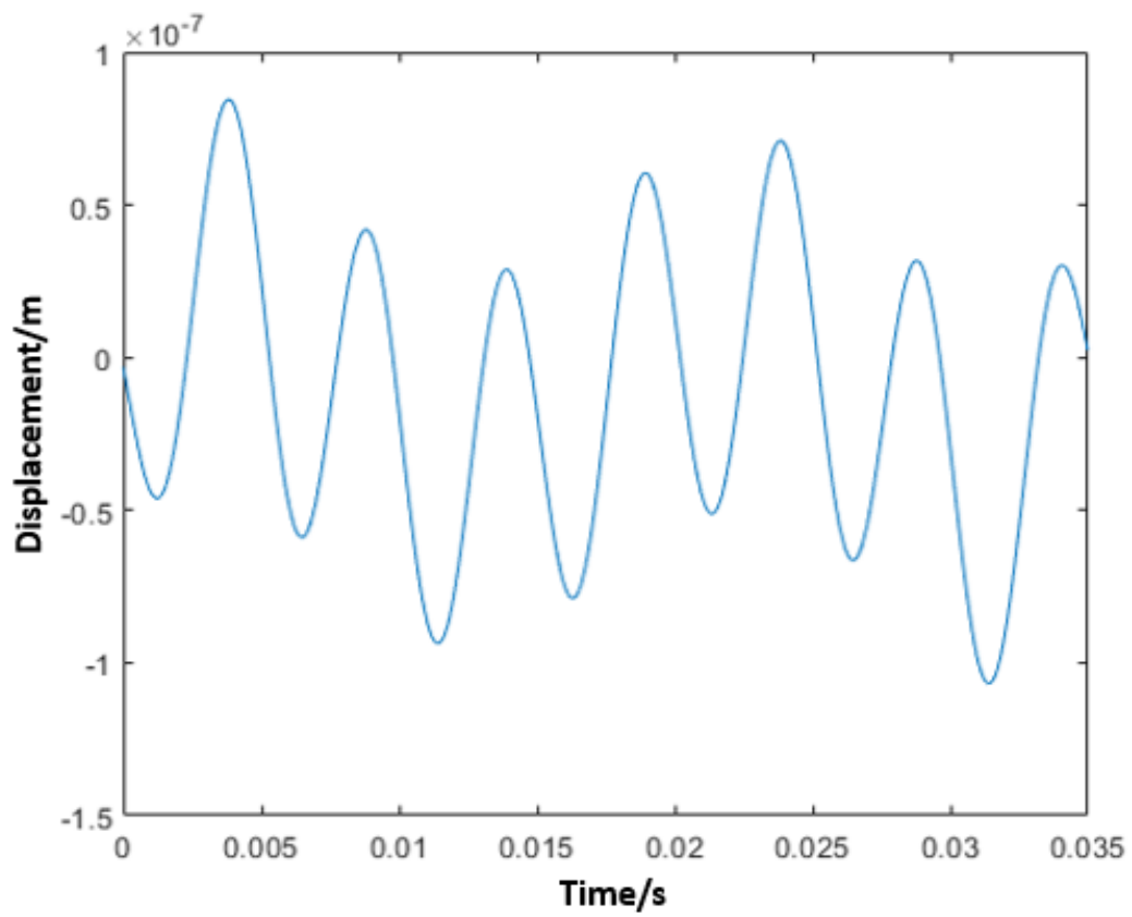
Figure. 5.10 The displacement data obtained using the double integration method and the acceleration data with the bias removed and the Butterworth filter applied.
