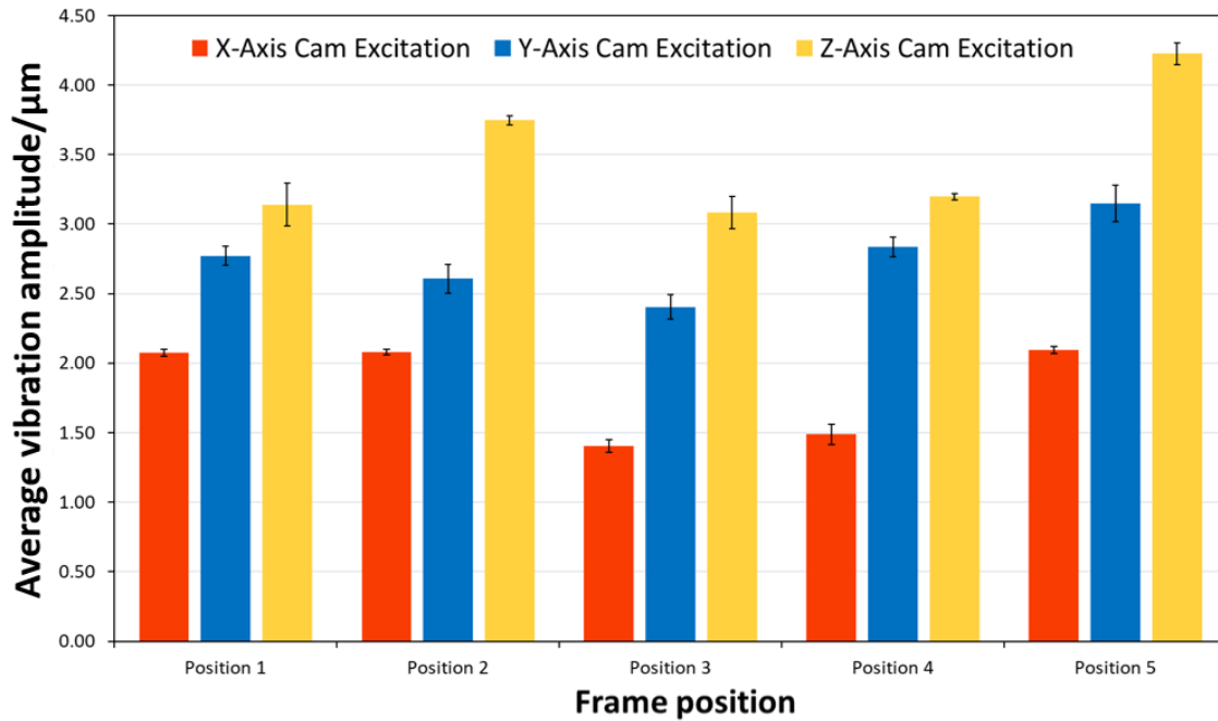
Figure. 5.16 Full frame three axis characterisation results in 5 key positions with the frame excited by a DSLR camera.
