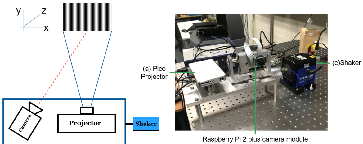
Figure. 4.5 Schema and picture of the combined vibrating experimental setup using an (a) iCODIS G1 pico projector (b) Raspberry Pi 2 with an 8 MP camera module, and (c) Smart Shaker K2007E01 which provides the vibration to the setup
