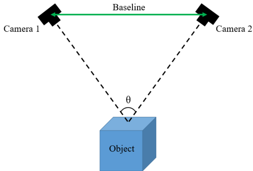
Figure. 2.3 The experimental configuration for photogrammetry, which uses two cameras to measure the form of an object by finding correspondence between the two captured images and triangulation to find the height of each point.
