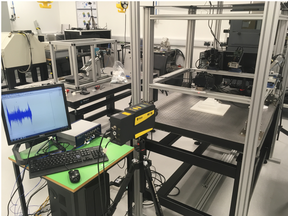
Figure. 5.18 The experimental setup using the Polytec portable digital laser vibrometer (PDV-100) to characterise the multi-view fringe projection mechanical system in order to verify the measured accelerometer results.
