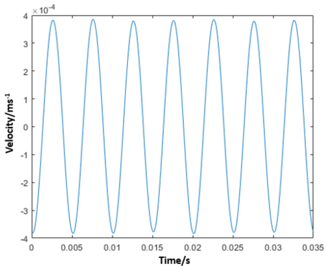
Figure. 5.11 The velocity data obtained using the omega arithmetic method to convert the acceleration data with a Butterworth filter applied.
