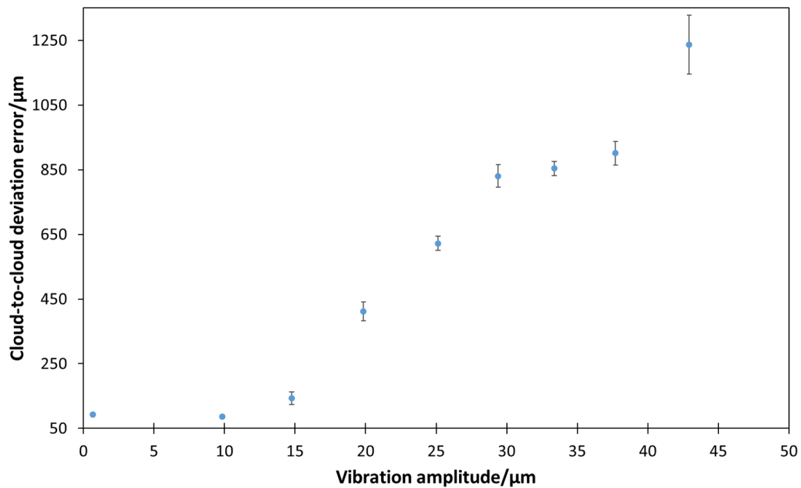
Figure. 7.15 A plot of increasing the amplitude of vibration in the y-axis against the mean cloud-to-cloud measurement error shows a significant rise in measurement errors as the captured images are increasingly blurred.
