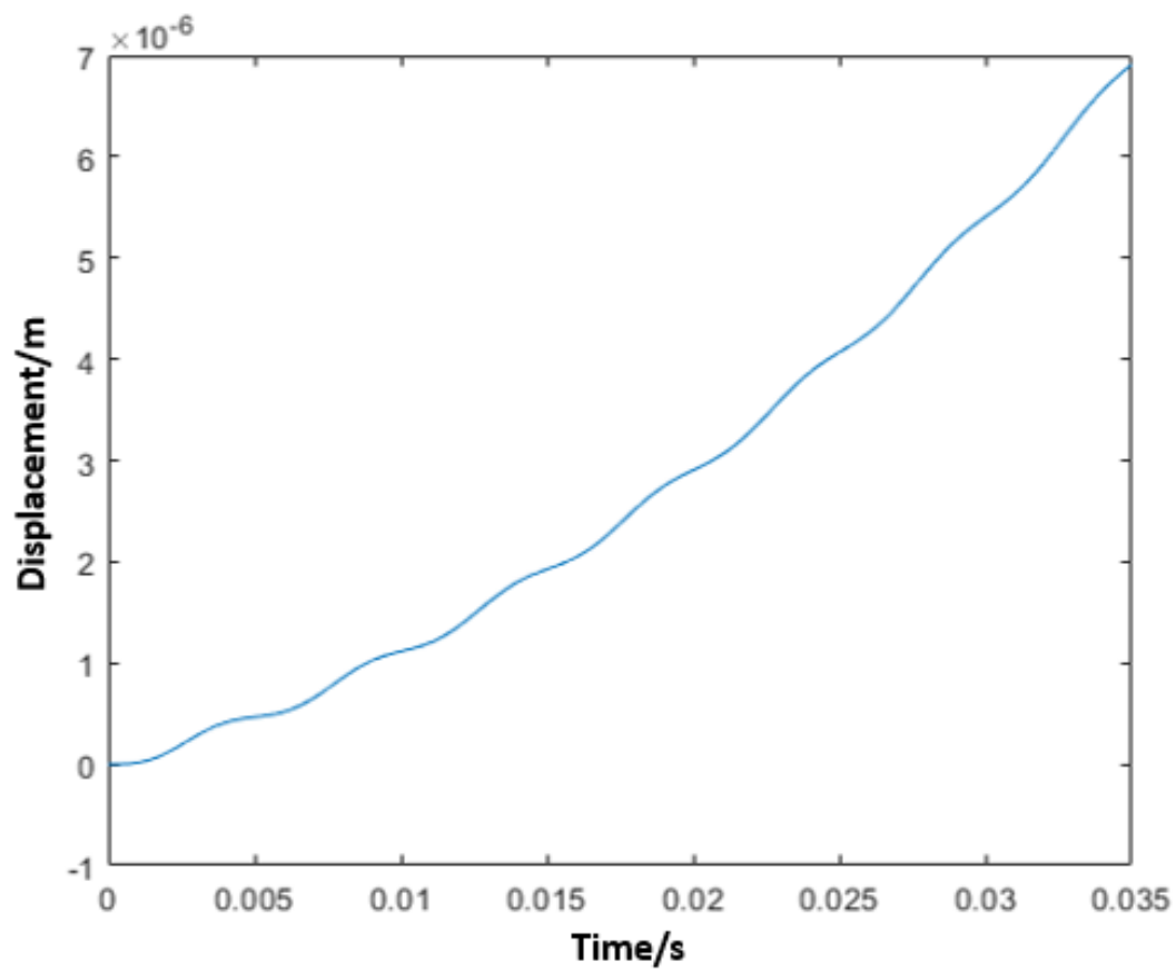
Figure. 5.7 The displacement dataset obtained using the raw measured z -axis acceleration data of a 200 Hz sinusoidal signal and the double integration method to convert to displacement.
