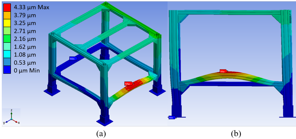
Figure. 4.18 Heat map results, (a) isometric view and (b) side view, of the maximum deformation on the complete frame assembly with the camera excitation applied to the frame in the z -axis, showing how the camera excitation in the middle of the horizontal strut would propagate around the structure.
