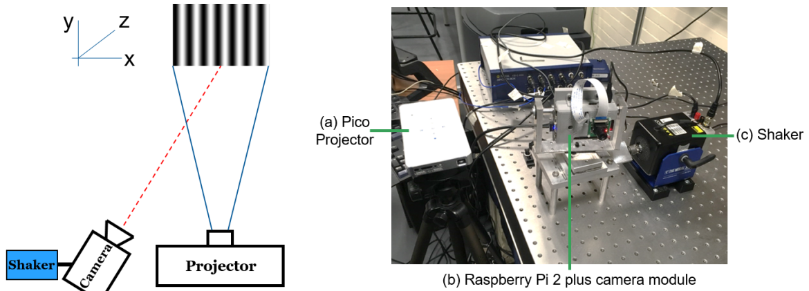
Figure. 4.3 Schema and picture of the camera vibrating isolated experimental setup using an (a) iCODIS G1 pico projector (b) Raspberry Pi 2 with an 8 MP camera module, and (c) Smart Shaker K2007E01 which provides the vibration to the setup
