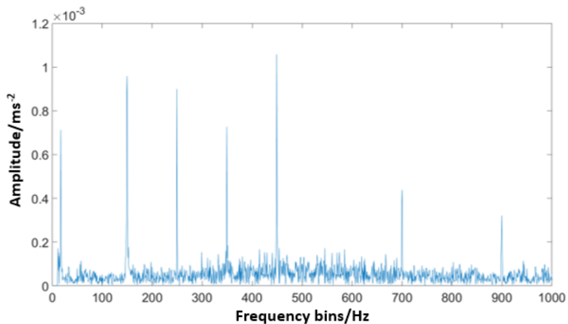
Figure. 5.17 The frequency response of the background vibration used to identify the different components of the signal, such as excitation from motorised equipment, machinery and road traffic.
