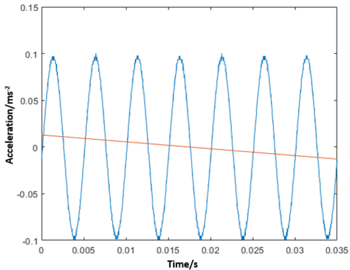
Figure. 5.8 The measured acceleration data after the bias (red line) has been removed and a Butterworth passband filter of 30 Hz to 1600 Hz has been applied to the measured accelerometer z -axis data.
