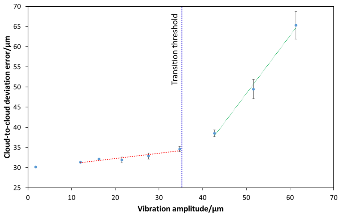
Figure. 7.6 A plot of increasing the amplitude of vibration in the y-axis against the mean cloud-to-cloud measurement error showing a sharp increase in the linear trend between the red and green dashed lines, which is due to the significant measurement errors seen around the edges of the complex features on the artefact. The blue dashed line shows the defined acceptable measurement threshold at the point the trends change.
