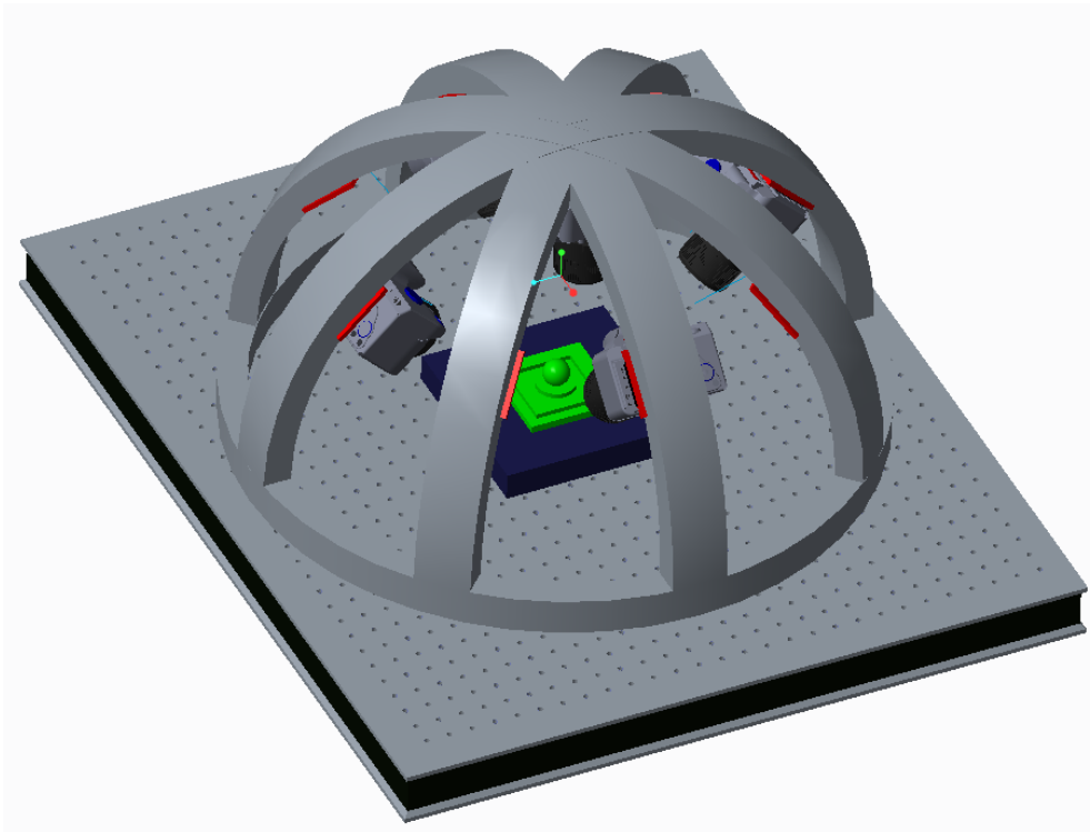
Figure. 4.12 CAD representation of the fourth concept ('circular arcs frame') proposed as a design solution for the multi-view fringe projection system.
