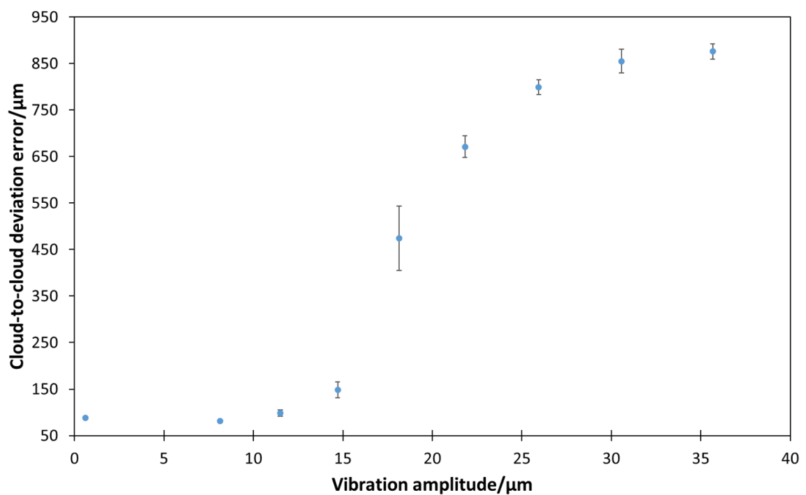
Figure. 7.11 A plot of increasing the amplitude of vibration in the x -axis against the mean cloud-to-cloud measurement error shows a significant rise in measurement errors as the captured images are increasingly blurred.
