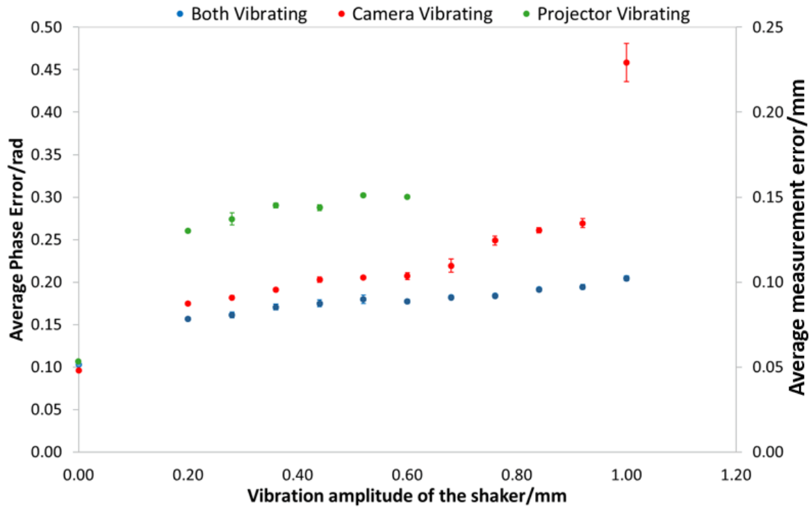
Figure. 4.7 Experimental results showing, increasing the amplitude of vibration on three experimental fringe projection setups causes an increase in mean measurement error.
