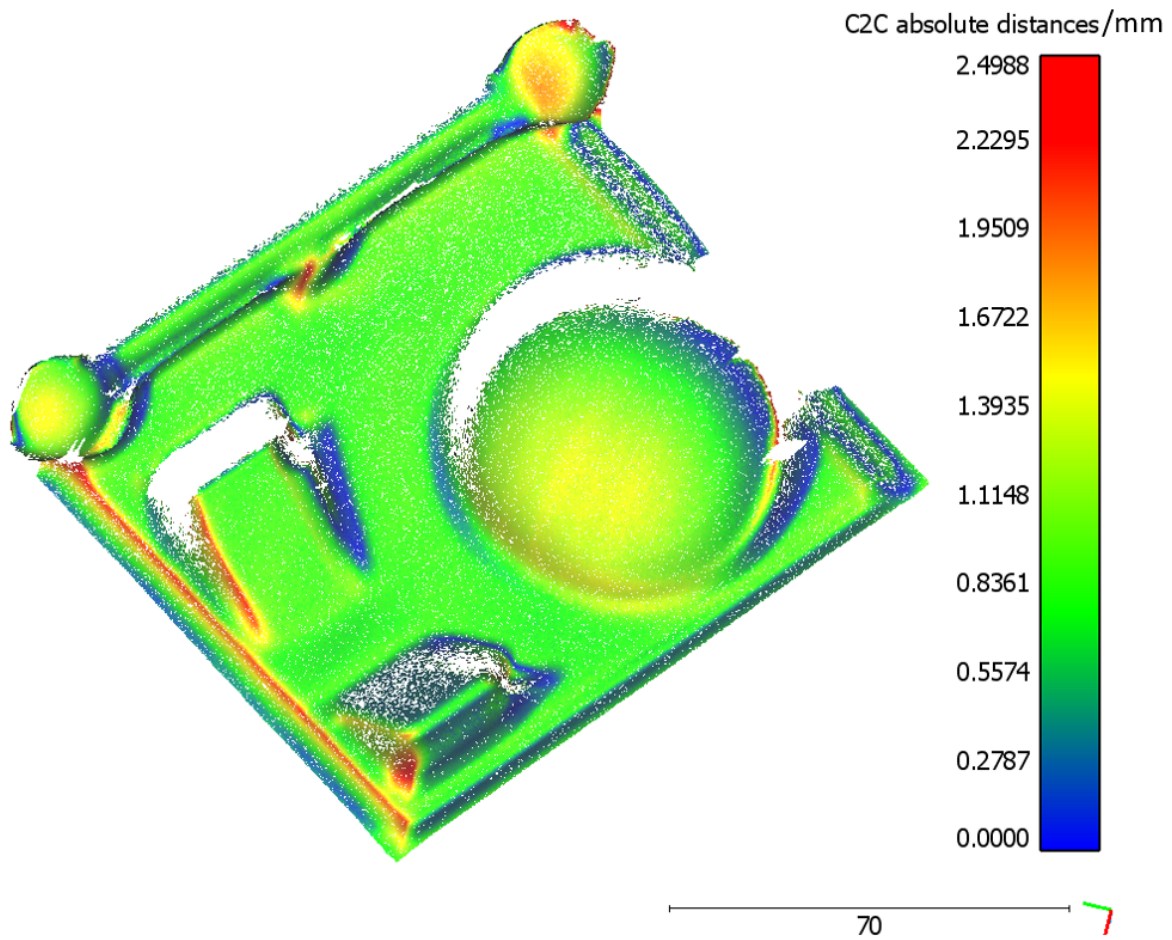
Figure. 7.14 Heat map of the cloud-to-cloud error analysis for 0.35 V vibration input of the shaker in the x -axis, showing the large measurement errors around the edges of the artefact due to the 'over-smoothing' effect.
