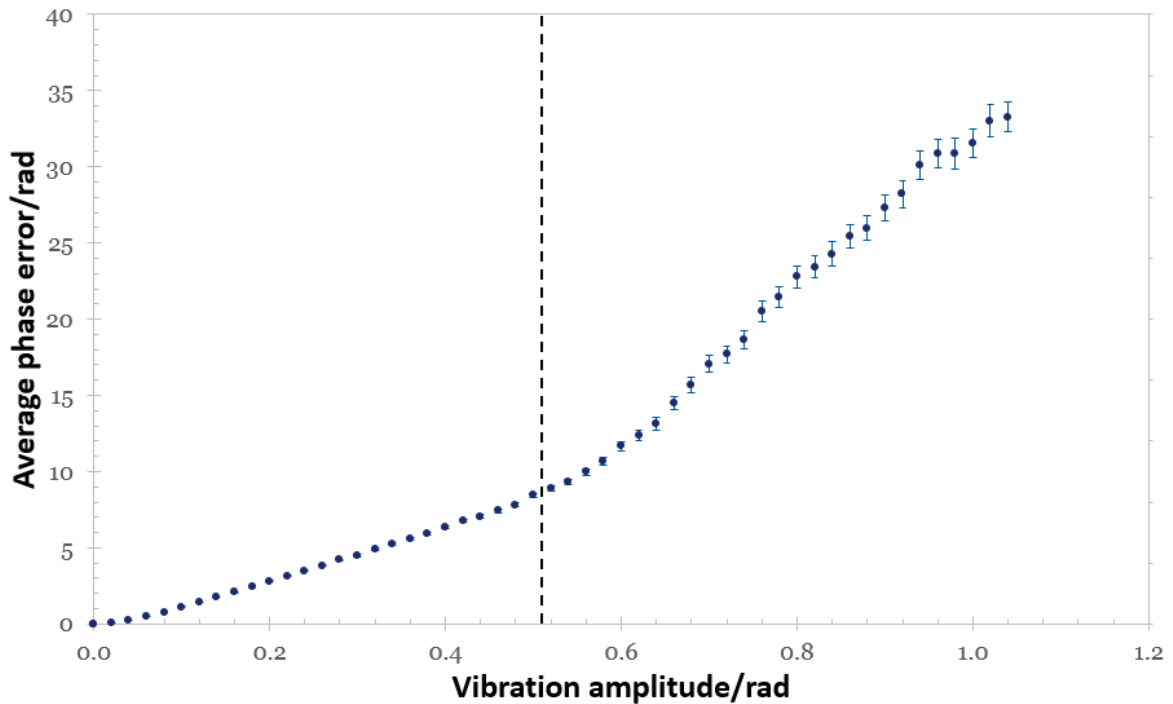
Figure. 4.2 Simulated results for the effects of vibration on fringe projection measurements, which shows increasing the amplitude of vibration causes an increase in the measured phase error, with a sharp increase in error seen when the amplitude exceeds the size of the phase shifts between patterns leading to phase unwrapping errors illustrated by the dashed line.
