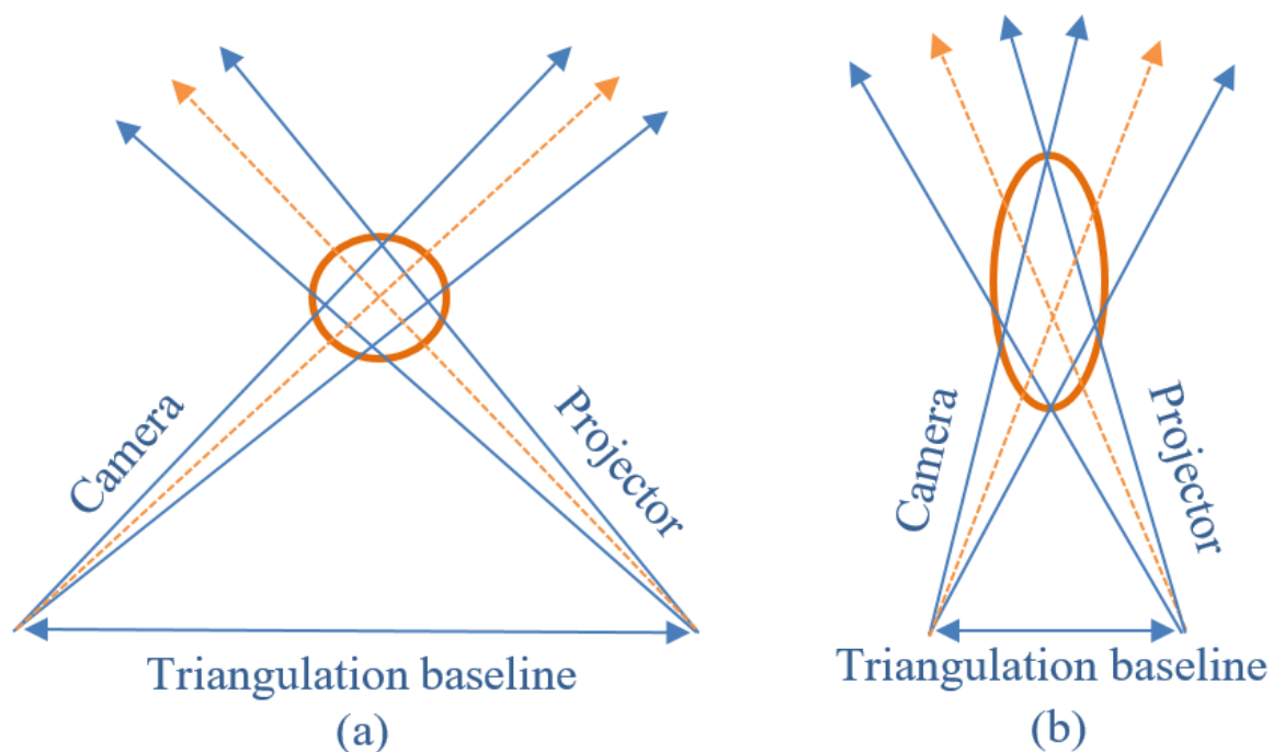
Figure. 2.10 Illustration of the projection errors caused by the uncertainty in the projection angles in both the camera and projector for both (a) wider baseline and (b) narrow baseline.
