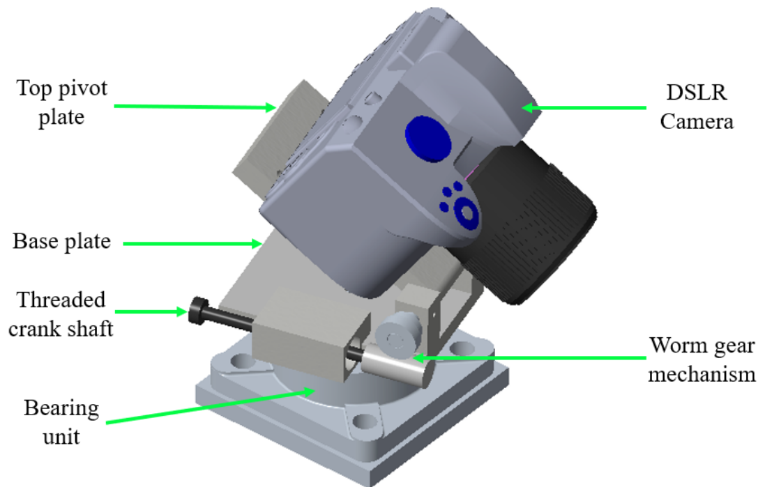
Figure. 4.20 CAD schematic of the camera mount design that was used in the multi-view fringe projection system.
