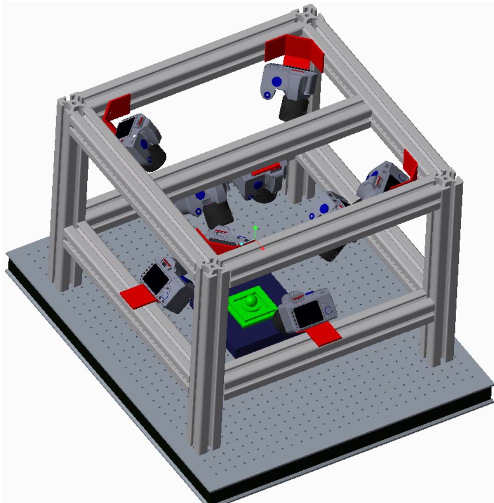
Figure. 4.10 CAD representation of the second concept ('rectangular item cage') proposed as a design solution for the multi-view fringe projection system.
