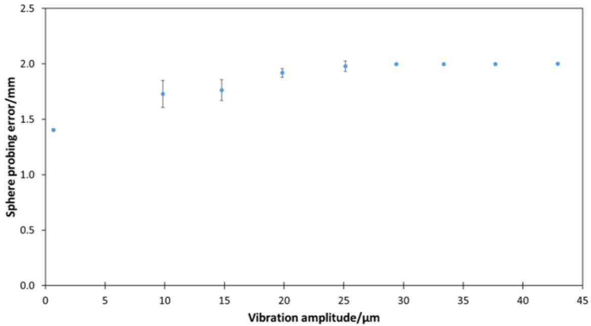
Figure. 7.16 A plot of increasing the amplitude of vibration in the y-axis against the sphere probing error (mean between the positive and negative) of a fitted sphere to the ball of the ball bar fixture on the AM artefact, shows the sphere probing error trend does not match the increasing measurement error.
