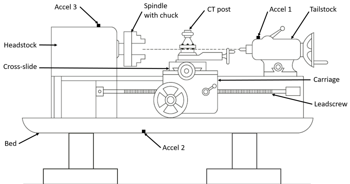
Figure. 6.10 Schema of the experimental configuration showing the key components of a lathe, and the accelerometer mounting positions for the condition monitoring investigation into the effects of the depth of cut and tool wear.
