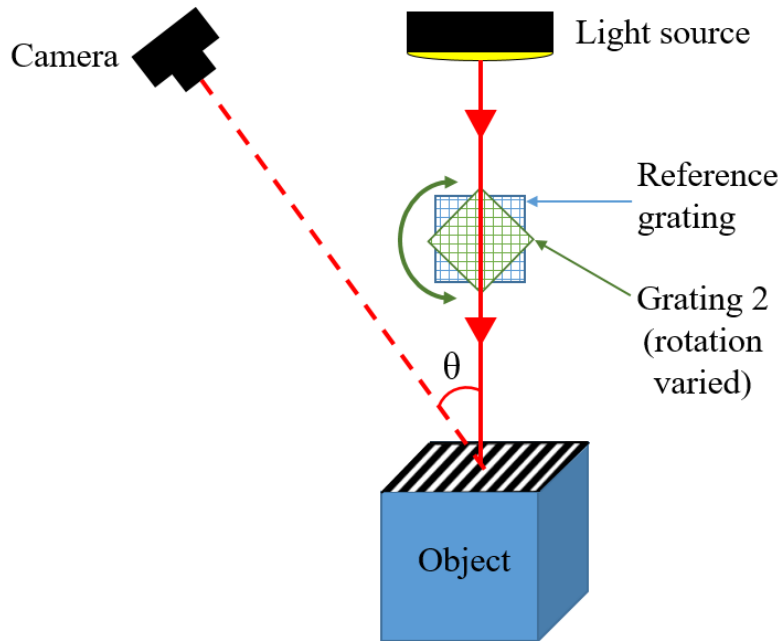
Figure. 2.5 The experimental configuration for Moiré fringe techniques, which uses two gratings to create the fringe patterns, and a camera to capture the pattern, which can be analysed to reconstruct the object's form.
