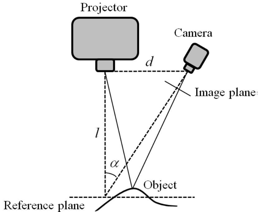
Figure. 2.6 Fringe projection system setup with one projector and one camera, the angles and baseline used for triangulation based fringe projection have also been illustrated [56].
