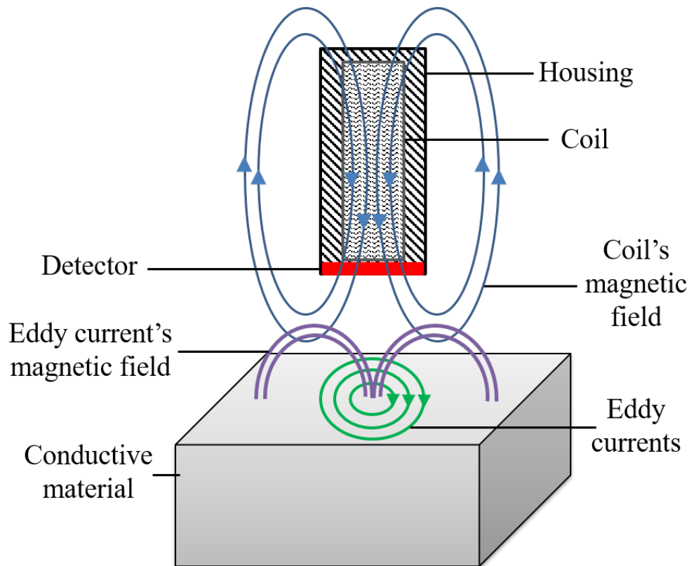
Figure. 5.1 Schematic diagram depicting the key elements of a proximity sensor.
