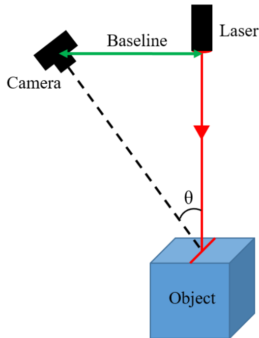
Figure. 2.2 The experimental configuration for laser scanning, which uses a laser and camera, and the principle of triangulation to measure the height of each point on the objects surface.
