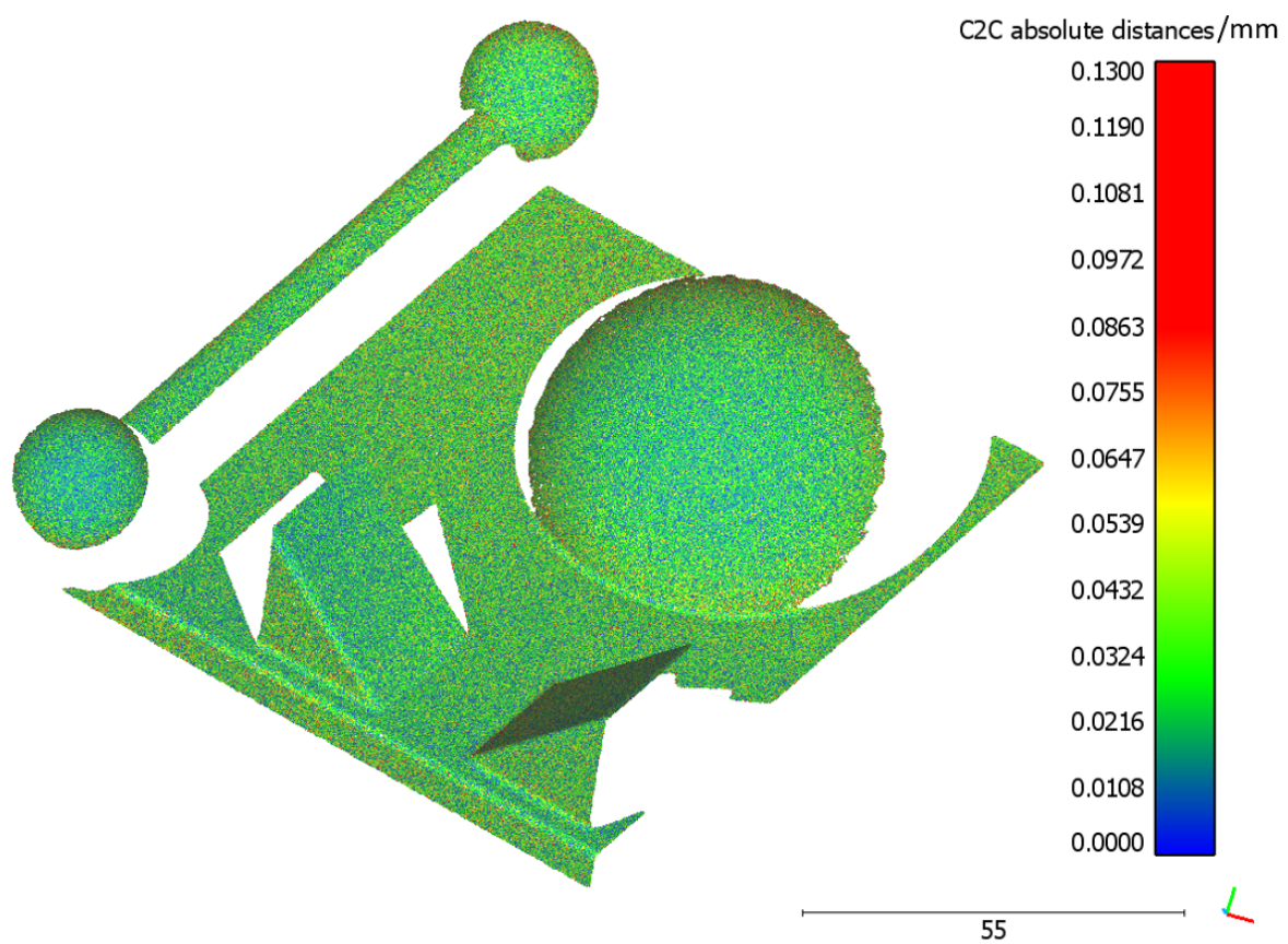
Figure. 7.4 Heat map of the cloud-to-cloud error analysis for 0.10 V vibration input of the shaker in the x -axis, showing the random distribution of errors across the measurement artefact.
