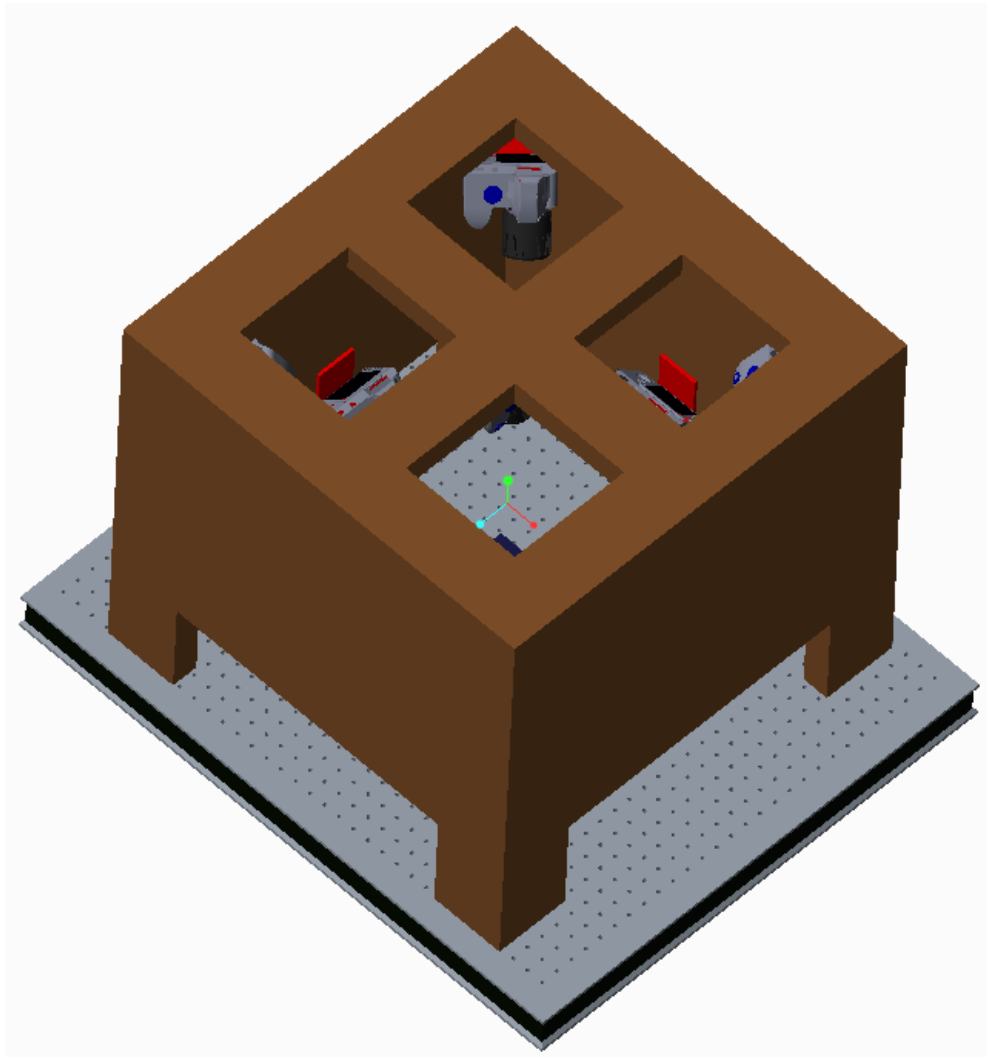
Figure. 4.11 CAD representation of the third concept ('one-piece frame') proposed as a design solution for the multi-view fringe projection system.
