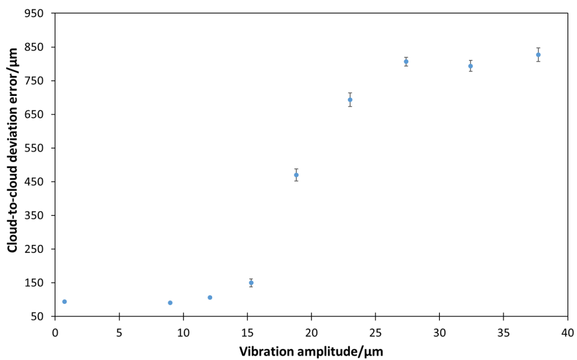
Figure. 7.17 A plot of increasing the amplitude of vibration in the z -axis against the mean cloud-to-cloud measurement error shows a significant rise in measurement errors as the captured images are increasingly blurred.
