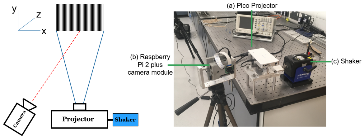
Figure. 4.4 Schema and picture of the projector vibrating isolated experimental setup using an (a) iCODIS G1 pico projector (b) Raspberry Pi 2 with an 8 MP camera module, and (c) Smart Shaker K2007E01 which provides the vibration to the setup
