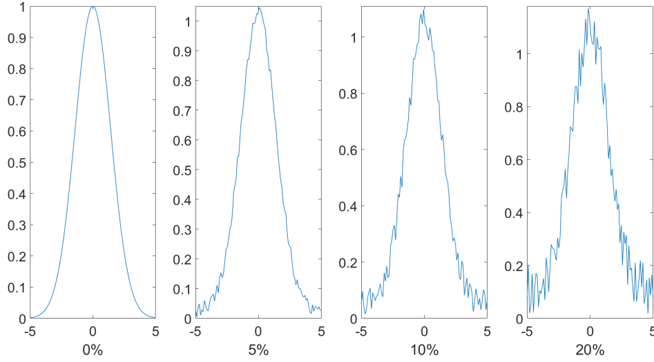
Figure. 2.11 Effect of noise on a point spread function. A noise level of 0%, 5%, 10% and 20% are shown.
