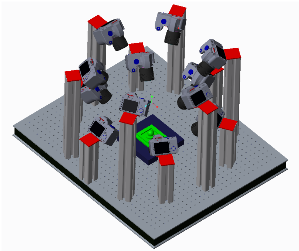
Figure. 4.9 CAD representation of the first concept ('individual posts') proposed as a design solution for the multi-view fringe projection system.
