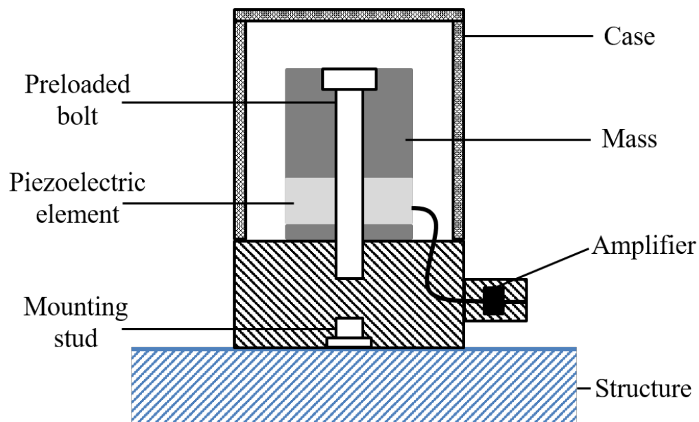
Figure. 3.2 Schematic diagram depicting the key elements of a piezoelectric accelerometer.
