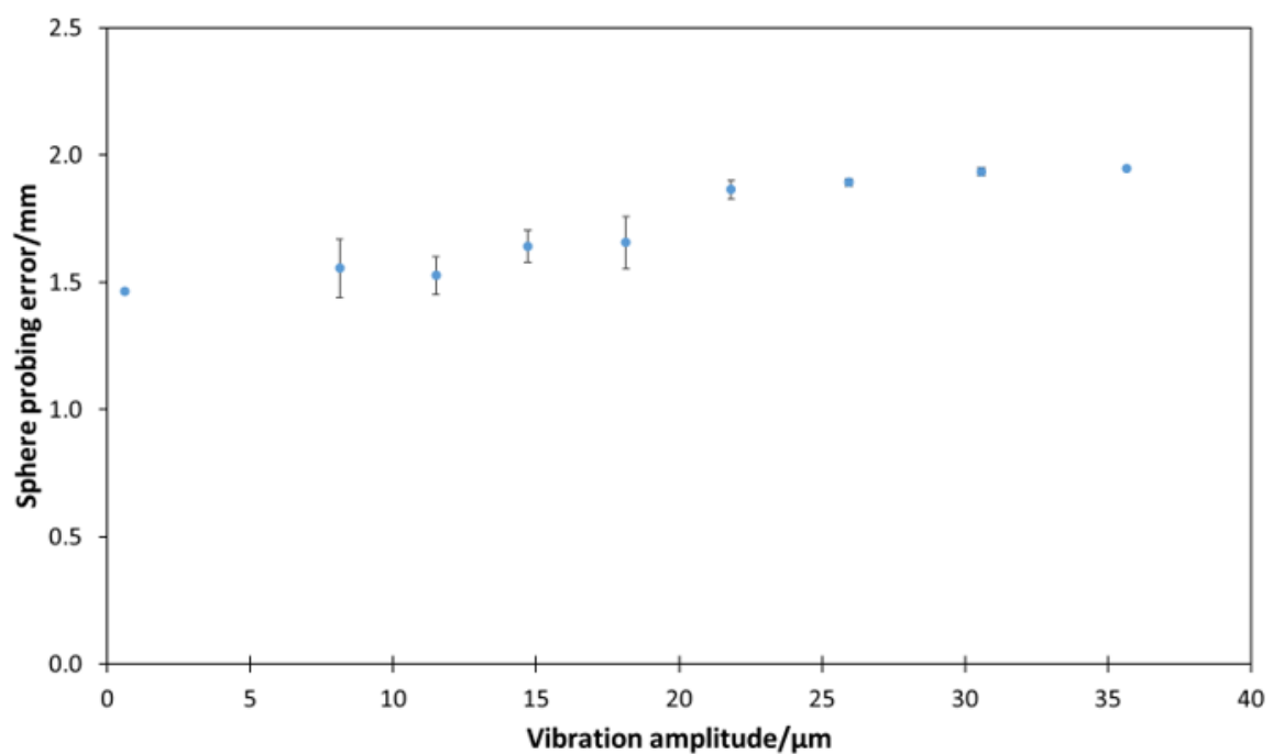
Figure. 7.12 A plot of increasing the amplitude of vibration in the x -axis against the sphere probing error (mean between the positive and negative) of a fitted sphere to the ball of the ball bar fixture on the AM artefact, shows the sphere probing error trend does not match the increasing measurement error.
