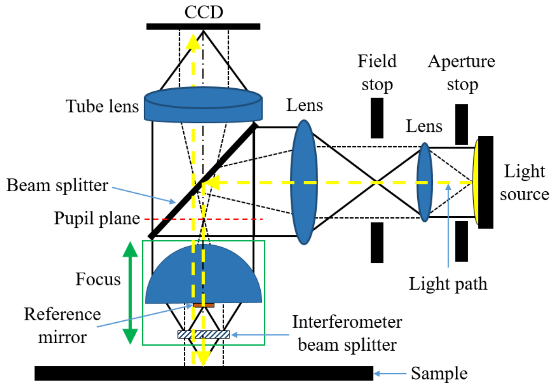
Figure. 2.4 The experimental configuration for interferometry, which reconstructs the object's surface by analysing the interference pattern created when the reference beam and measurement beam are superimposed.
