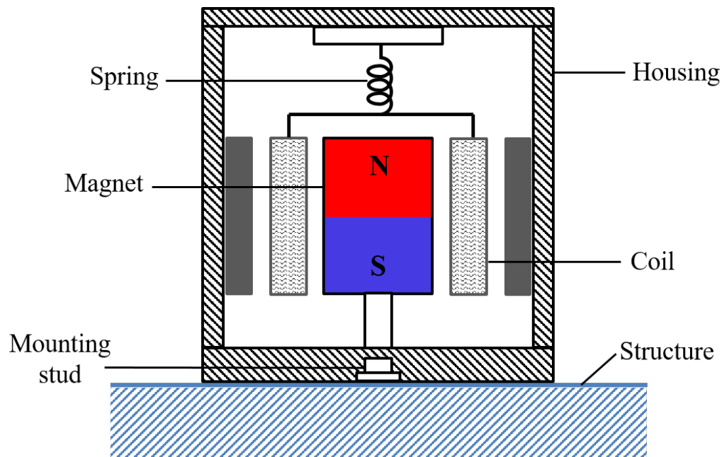
Figure. 5.2 Schematic diagram depicting the key elements of a velocity transducer.
