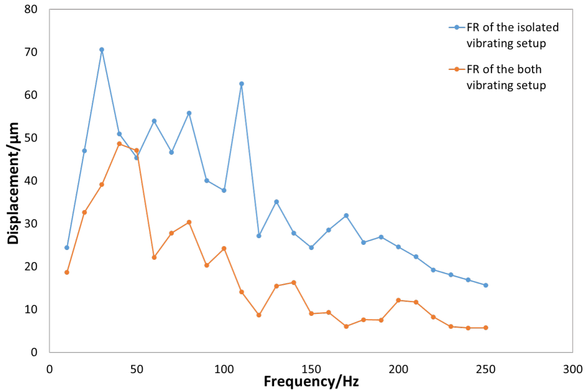
Figure. 4.6 Frequency response of both the isolated configuration and the combined configuration to varying vibration frequencies applied to the system, used to identify the natural frequency of the experimental setups.
