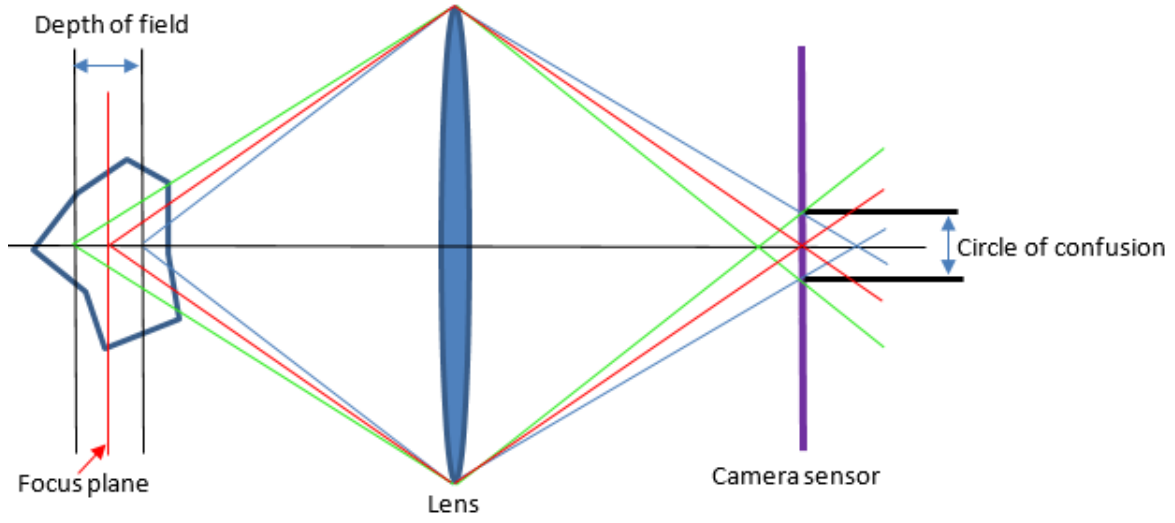
Figure. 2.9 Illustration of the principle behind the circle of confusion.
