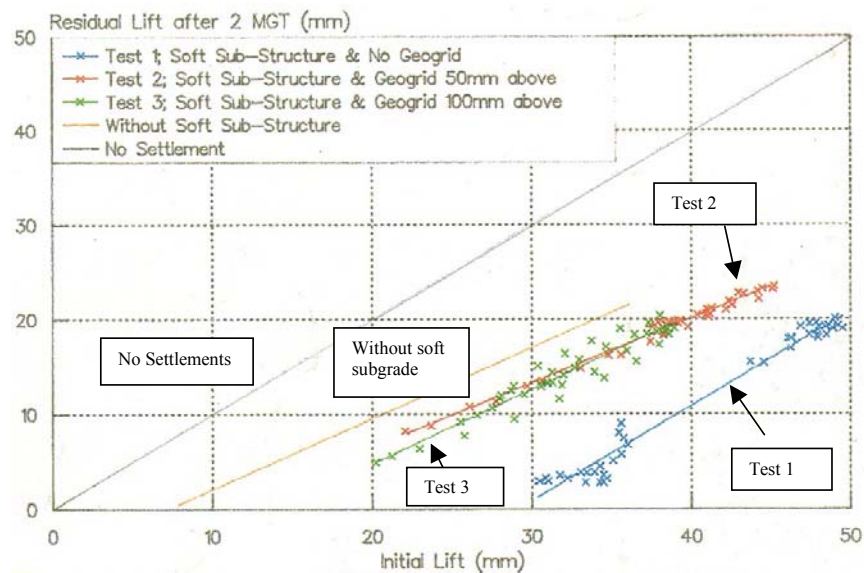
Figure 2.36 Initial Vs Residual Lift (Matharu, 1994)
