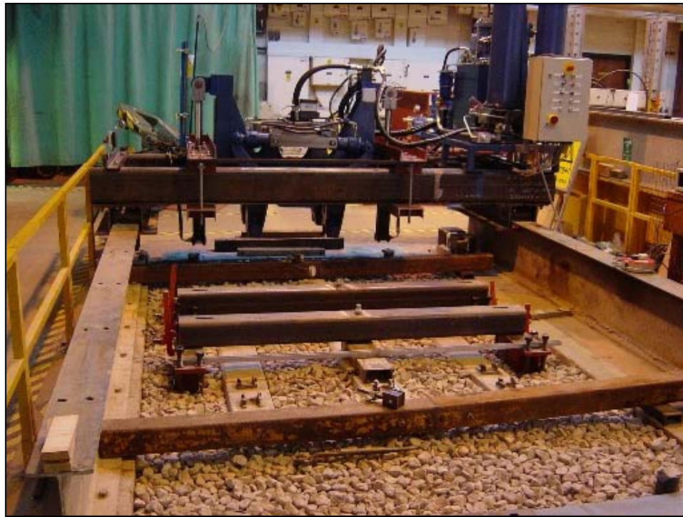
Figure 5.14 The tamping bank facility
