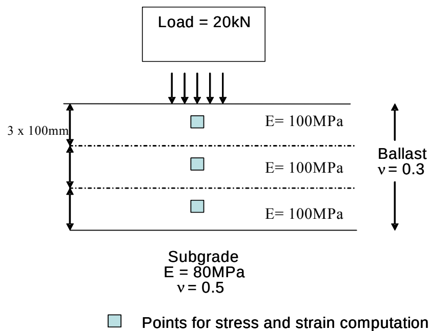
Figure 7.6 Structural details for CET analysis
