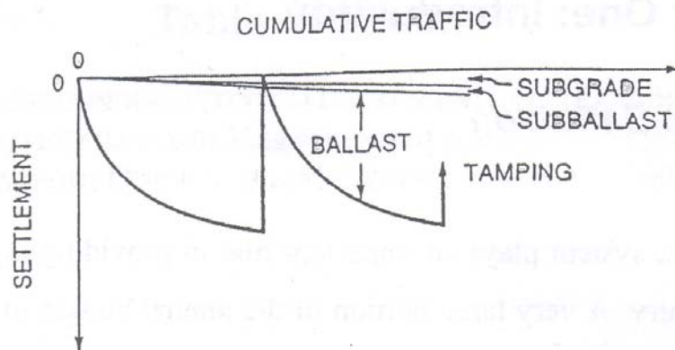
Figure 1.1 Substructure contributions to Settlement (Selig and Waters, 1994)
