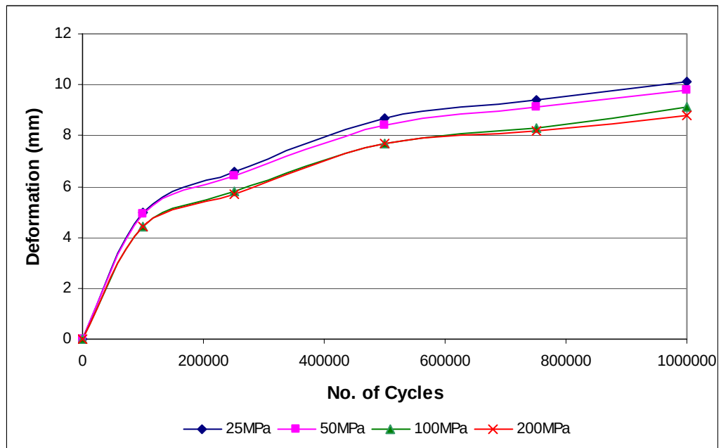
Figure 7.13 Influence of subgrade stiffness on computed settlement for unreinforced track
