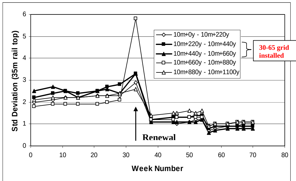
Figure 6.3 HSTRC Data
