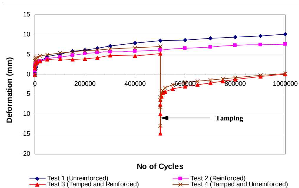
Figure 5.24 Settlement accumulations in the 4 RTF tests
