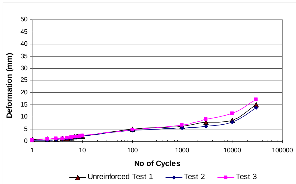
Figure 4.10 Control tests on stiff subgrade (unreinforced)
