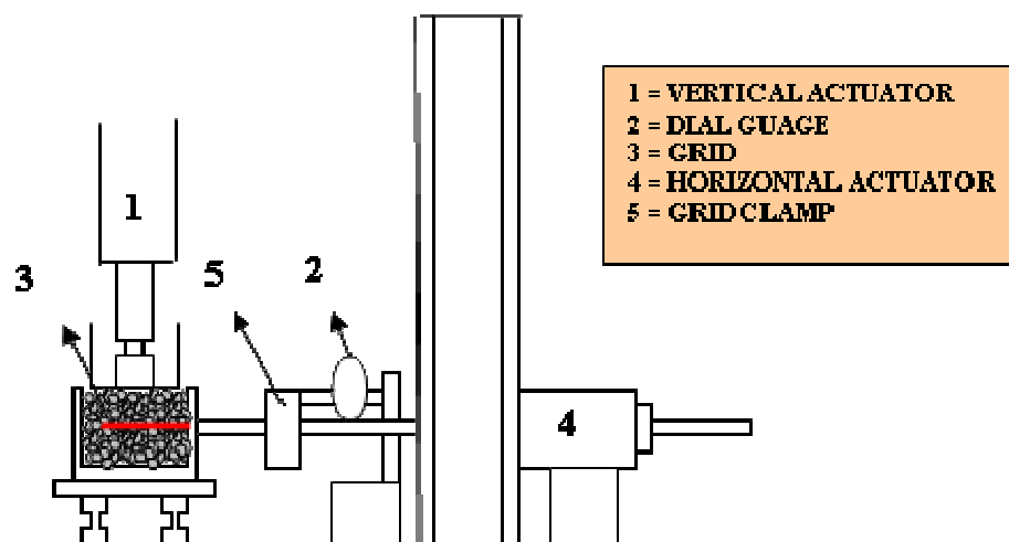
Figure 3.7 Schematic diagram of Pull-out Test
