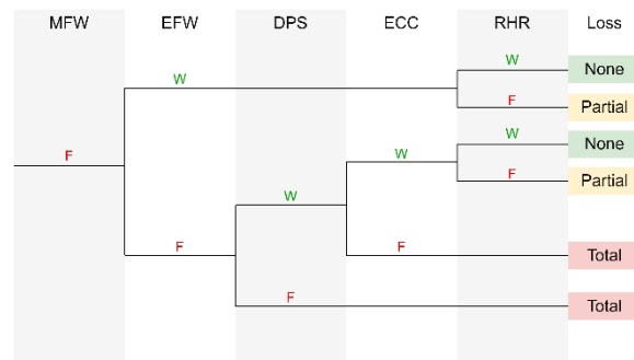
Figure 2 ET model of the loss of main feed water accident
